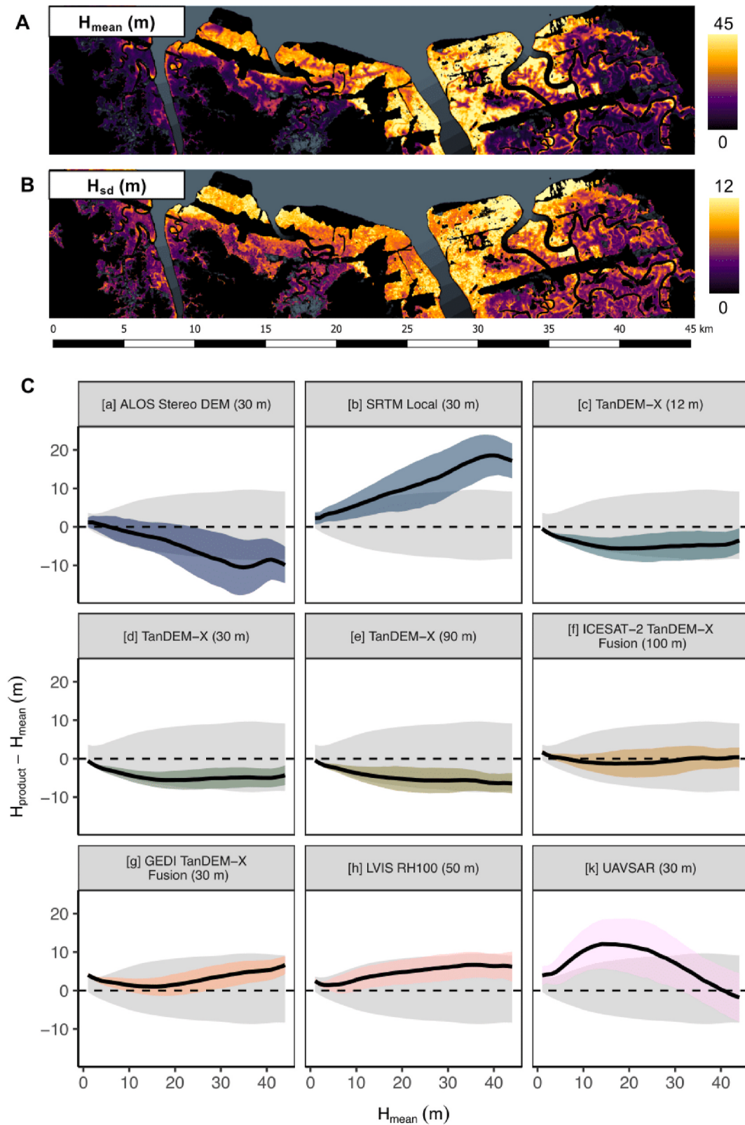
Fig. 5. (A) Example map of mean mangrove canopy height ( H_{\text{mean}} ) and (B) variation across the 9 sensors compared in this study. Relationship between sitewide mean mangrove canopy height ( H_{\text{mean}} ) and (C) product heights minus H_{\text{mean}} and standard deviation (within a product (color) and across products (grey)) from 9 remote sensing products. Variability increases with H_{\text{mean}} , while the equivalent relative variation decreases with H_{\text{mean}} (See Supplementary Material Fig. S3 ). (For interpretation of the references to color in this figure legend, the reader is referred to the Web version of this article.)
