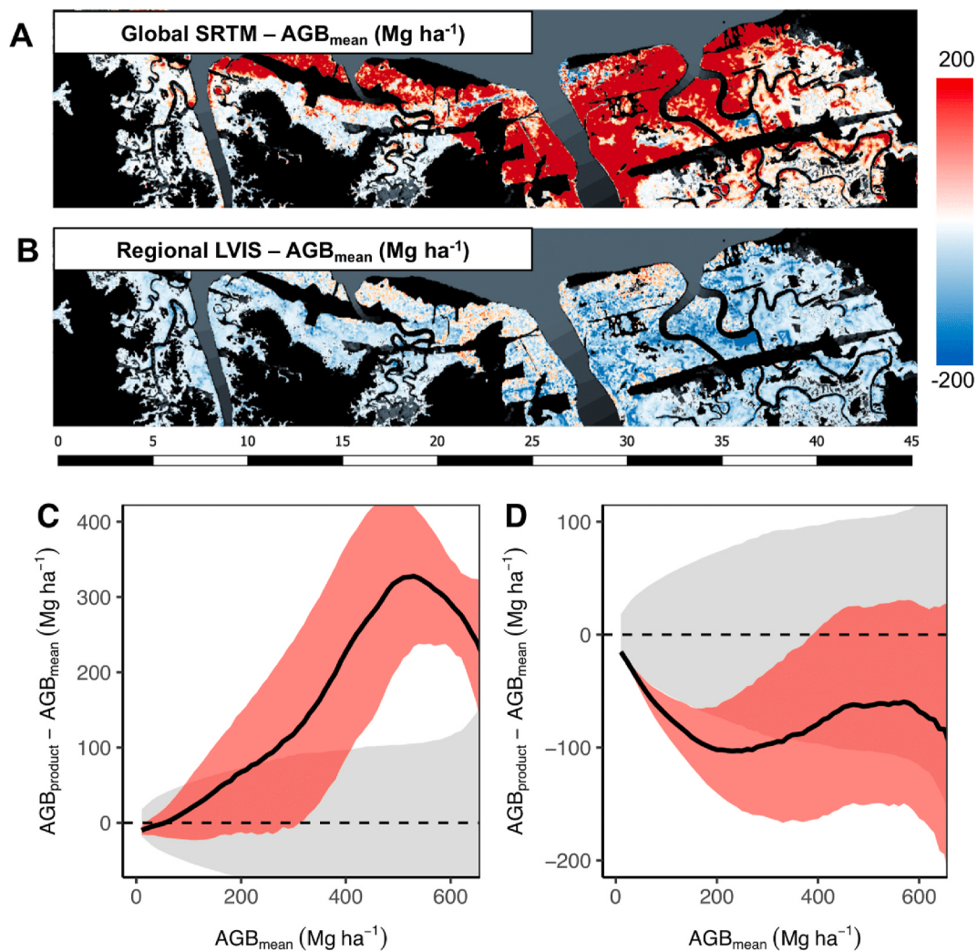
Fig. 8. Pixel-level comparison of local mean (across 9 products) aboveground biomass estimates (AGB mean ) and the [A] Global SRTM mangrove biomass and [B] regional LVIS biomass products. The residual plots indicate a systematic positive difference in the [C] SRTM-based model, increasing with increasing biomass values, and a systematic negative difference in the [D] regional LVIS biomass model.
