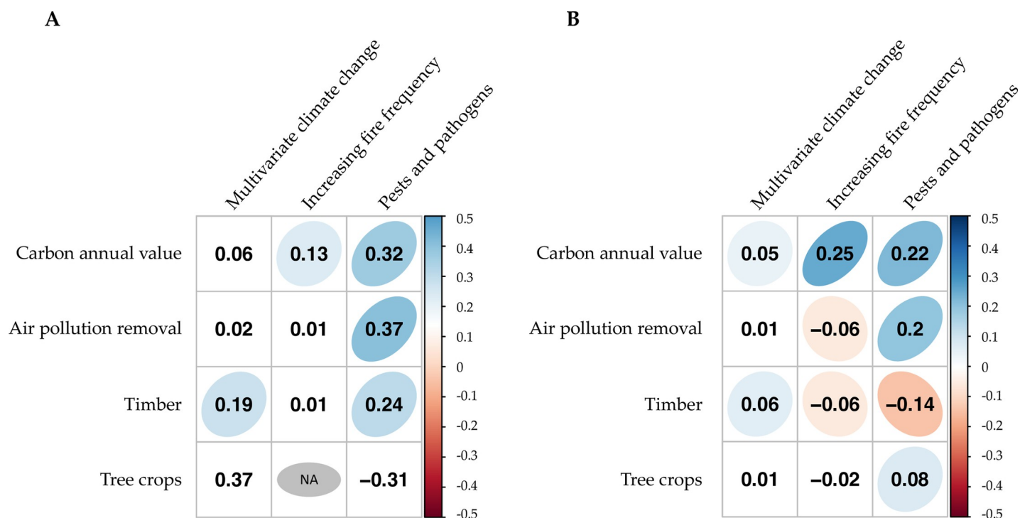
Fig 5. Associations between annual net ecosystem service values of tree species in the US and their predicted threats and drivers of change based on Spearman's rank-order correlations. A) Species-level correlation coefficients ( \rho ) between annual net ecosystem service value and predicted threats. B) Spatial correlations between annual net ecosystem service value and predicted threats by US counties. Colors (blue) indicate significant positive associations, indicating more valuable tree species are under more threat. Darker colors indicate stronger correlations. Service values refer to those generated between 2010 and 2012. Modeled expectations for changes in frequencies of major fire are not available in some regions precluding accurate estimation of their potential threat to some tree crop species in A; correlation is not shown.
