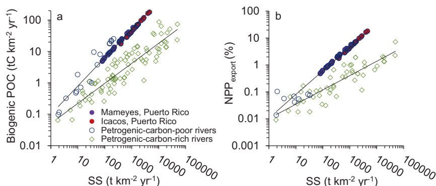
Fig. 2 River suspended load relationships for global rivers. The relationships are between a biogenic particulate organic carbon (POC) and b net primary productivity (NPP) export (%) relative to suspended sediment (SS) yield for global rivers.
