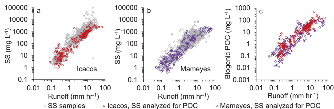
Fig. 1 River constituent concentrations in relation to runoff in the Luquillo Mountains. The relationship between river suspended sediment (SS \text{mg L}^{-1} ) relative to river runoff ( \text{mm hr}^{-1} ) for a Icacos and b Mameyes, with SS samples analyzed for particulate organic carbon (POC)% represented by colored circles. c Relationship between measured biogenic POC ( \text{mg L}^{-1} ) relative to runoff. Biogenic POC ( \text{mg L}^{-1} ) was estimated from SS samples that were not measured for POC% (gray circles) using Eq. 5 for Icacos and Eq. 6 for Mameyes.
