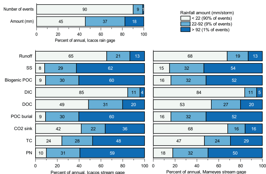
Fig. 3 Percent contribution of annual runoff and river exports by rainfall event size for the Icaicos and Mameyes Rivers. These exports are separated by rainfall amount as a percentage of annual total (SS suspended sediment, POC biogenic particulate organic carbon, DIC dissolved inorganic carbon, DOC dissolved organic carbon, POC burial estimated POC burial in ocean if biogenic POC burial efficiency is estimated at 22% 28 , CO2 sink estimated atmospheric carbon sink (POC burial + DIC), TC total carbon (POC + DIC + DOC), PN particulate nitrogen).
