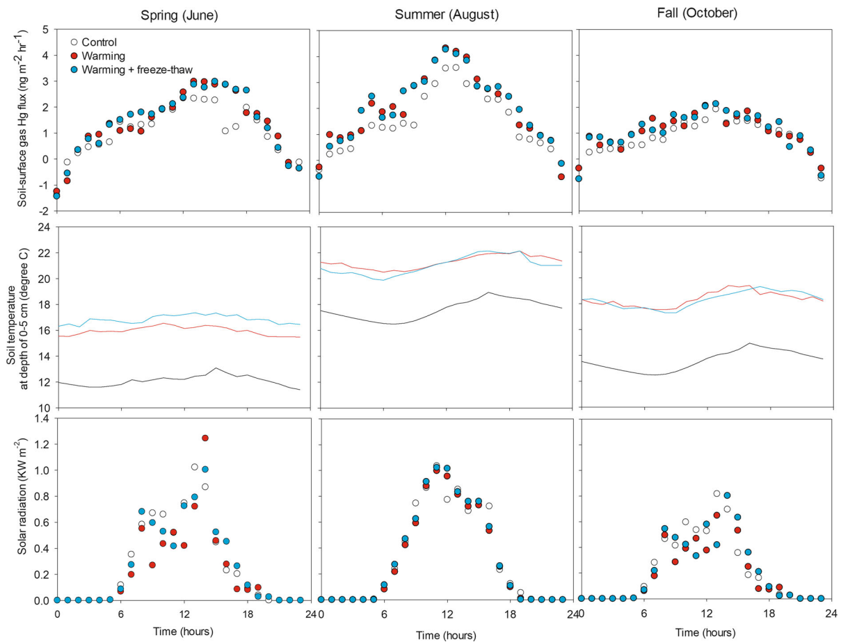
Fig. 1 Soil Hg 0 evasion and soil temperature and solar radiation at soil warming, soil warming + freeze-thaw cycles, and control plots across the three sampling dates
