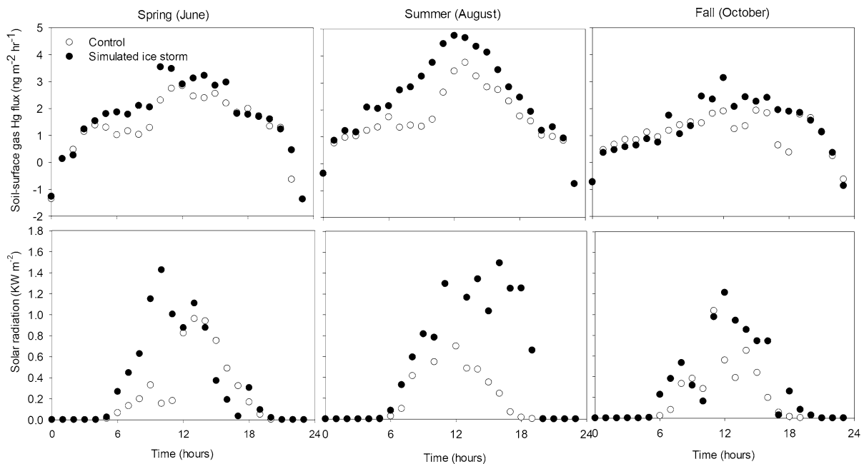
Fig. 2 Soil \text{Hg}^0 evasion was stimulated following a simulated ice storm at three sampling dates. Solar radiation was also higher in the plot with the simulated ice storm
