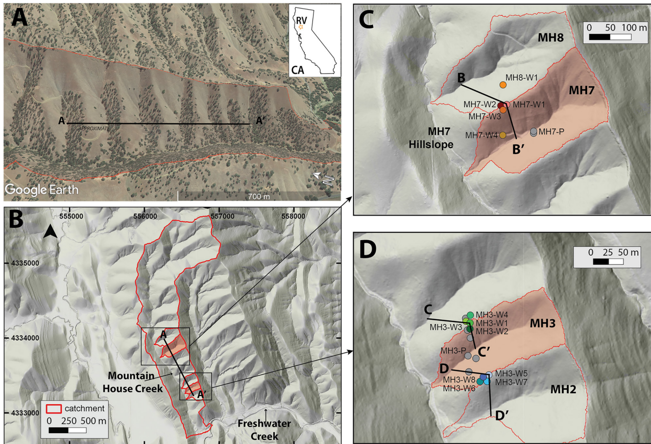
Figure 1. (a) Google Earth image of the study site (with terrain height-scaled 2×), where the red outlines delineate the Mountain House catchment and subcatchments where boreholes and monitoring infrastructure are located. (b–d) LIDAR-derived hillshade maps of the study site, with “c” and “d” zoomed in to the MH7 and MH3 hillslopes (respectively) and include borehole locations and cross-sections lines, which are used to illustrate hillslope profiles in Figure 3. Modified from Pedrazas et al. (2021).
