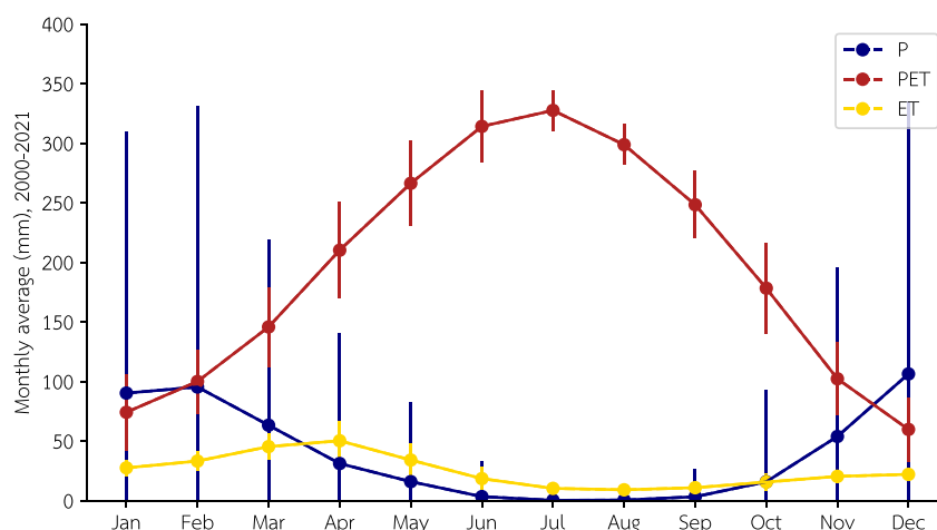
Figure 2. Composite annual timeseries of mean monthly precipitation (P), potential evapotranspiration (PET), evapotranspiration (ET) at Rancho Venada for the period 2000–2021. P is from PRISM dataset AN81d, and PET and ET are from the MODIS dataset MOD16A2. Errorbars represent one standard deviation.
