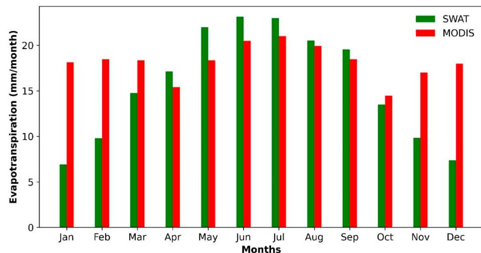
Figure 8. Comparison of long-term monthly SWAT-simulated vs. MODIS evapotranspiration data.
