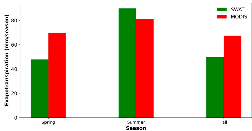
Figure 10. Comparison of long-term average seasonal SWAT-simulated vs. MODIS evapotranspiration data.
