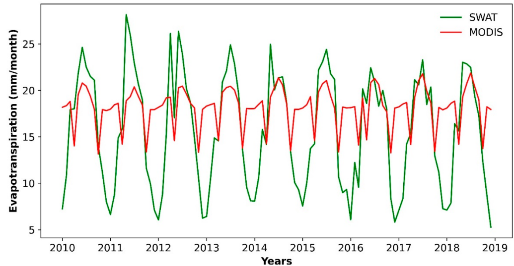
Figure 7. Comparison of monthly SWAT-simulated vs. MODIS evapotranspiration data.
