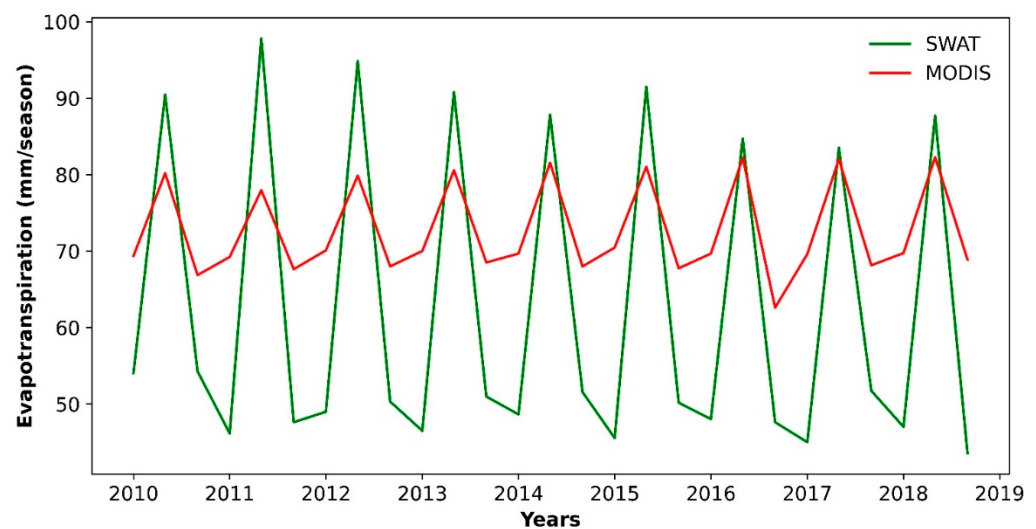
Figure 9. Comparison of seasonal SWAT-simulated and MODIS evapotranspiration data.
