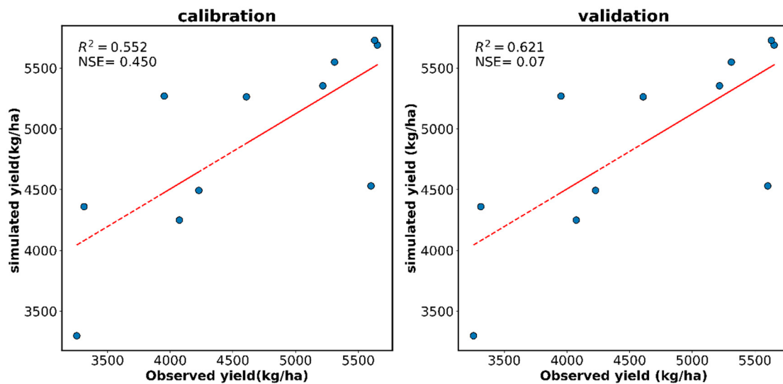
Figure 5. Comparison of observed vs. simulated annual soybean yield during model calibration and validation.
