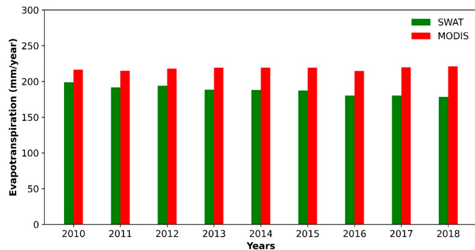
Figure 11. Comparison of annual SWAT-simulated vs. MODIS evapotranspiration data.
