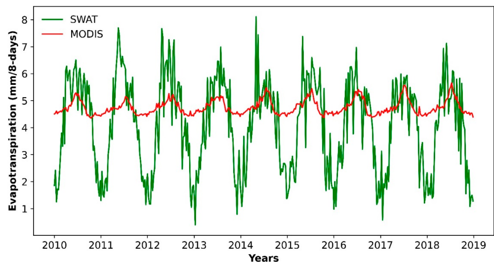
Figure 6. Comparison of 8-day SWAT-simulated vs. MODIS evapotranspiration data.
