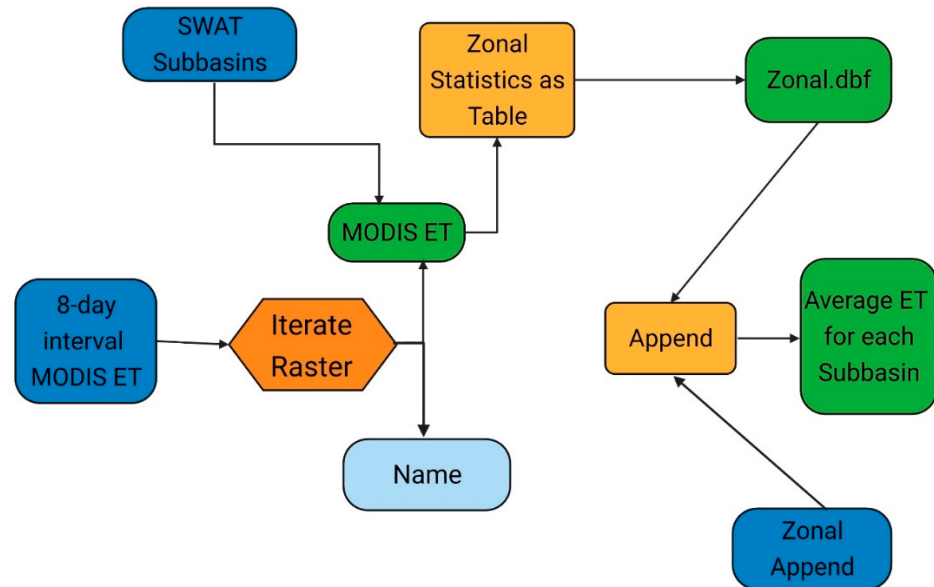
Figure 3. GIS-based model schematic to obtain average sub-basin-level MODIS evapotranspiration data for the watershed.
