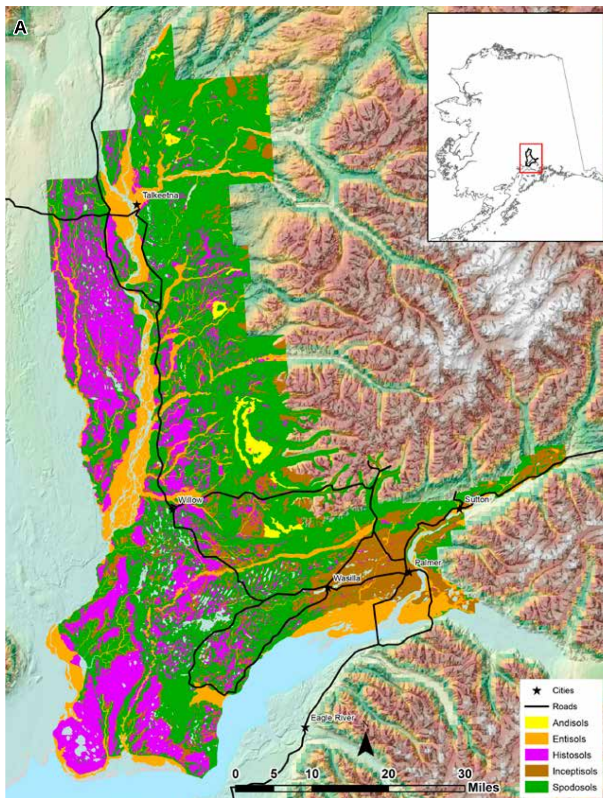
Figure A.2—Soil taxonomy order in the (A) Matanuska-Susitna Valley area and (B) western Kenai Peninsula survey areas (USDA NRCS 2019a, 2019b.).
