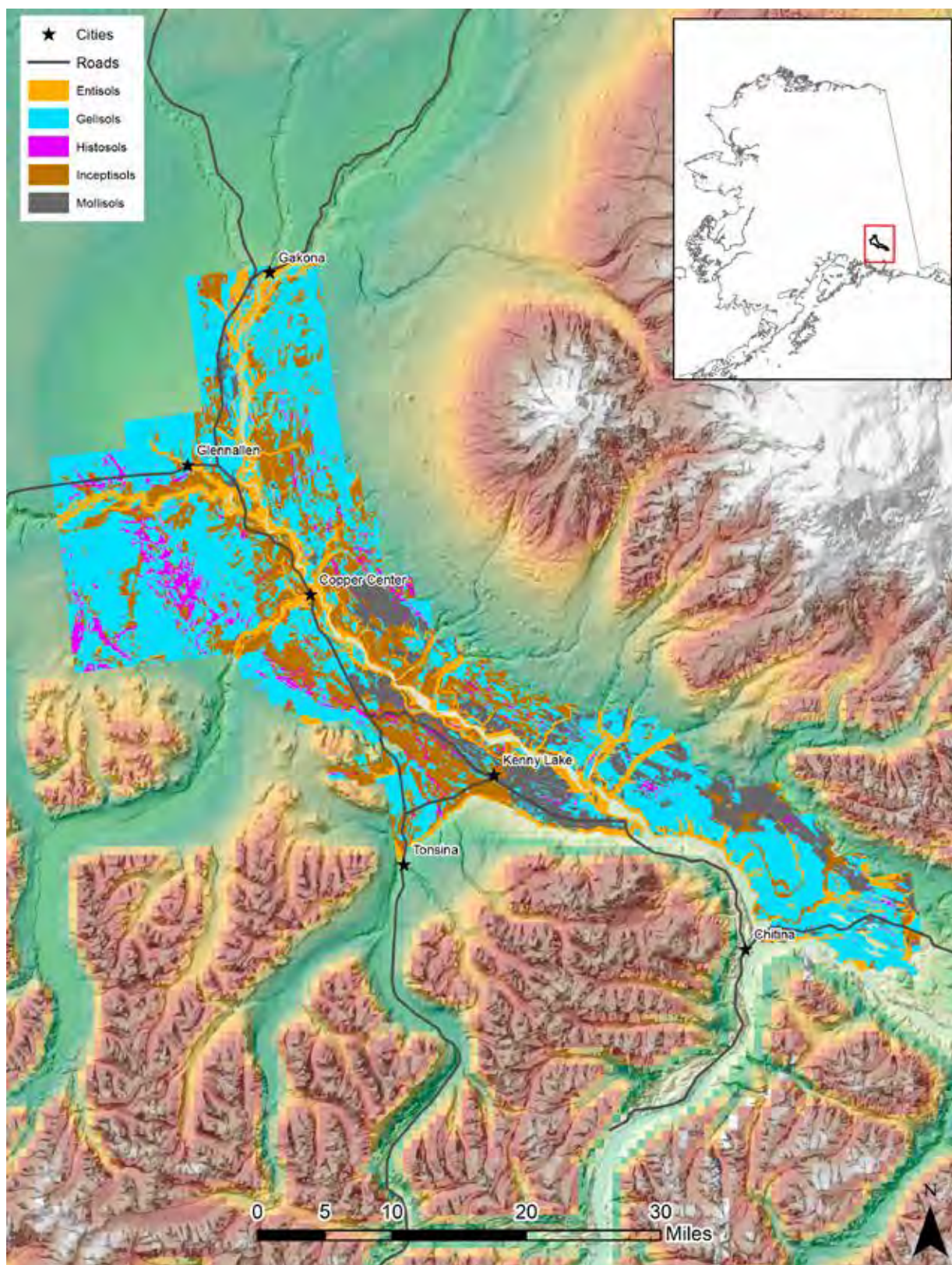
Figure 1.7—Soil taxonomy orders (Entisols = orange, Gelisols = blue, Histosols = purple, Inceptisols = brown, and Mollisols = grey) in the Copper River Valley survey area (USDA NRCS 2019c).
