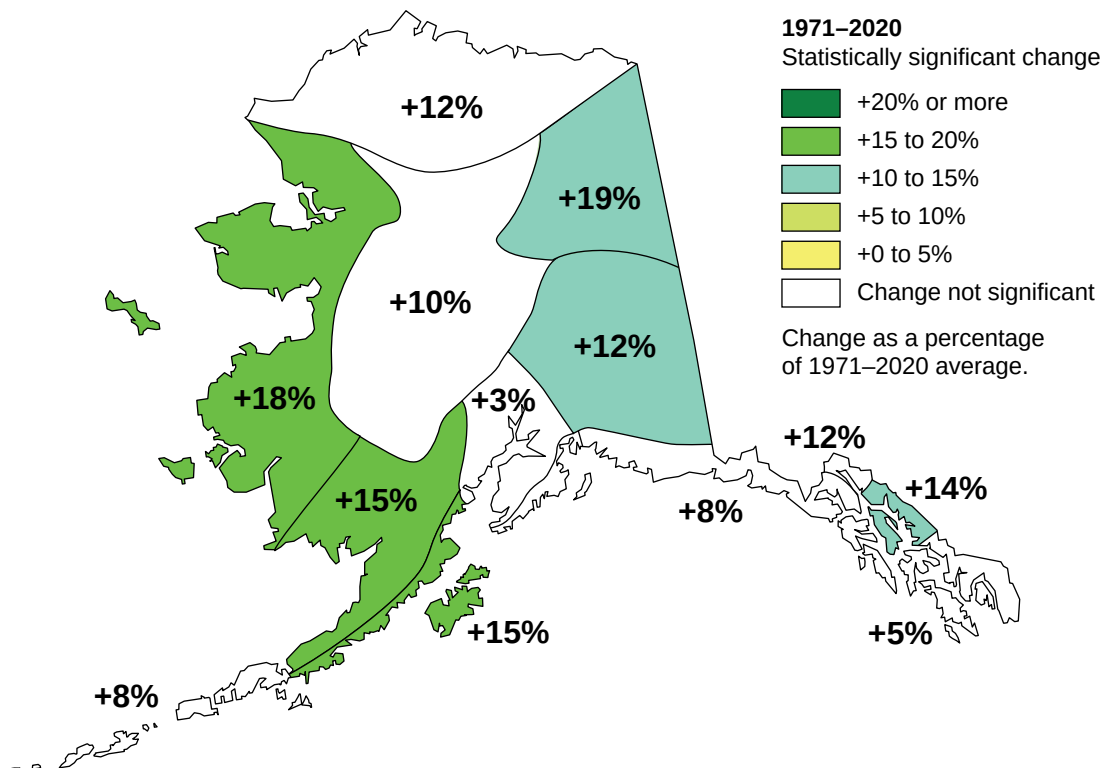
Figure 1.4—Some areas in Alaska have experienced increases in annual precipitation over the past 50 years as indicated by the colored regions. Increases in precipitation have varied by National Oceanic and Atmospheric Administration (NOAA) climate divisions. Only colored regions had statistically significant changes in precipitation. Data source: NOAA and National Centers for Environmental Information (NCEI).
