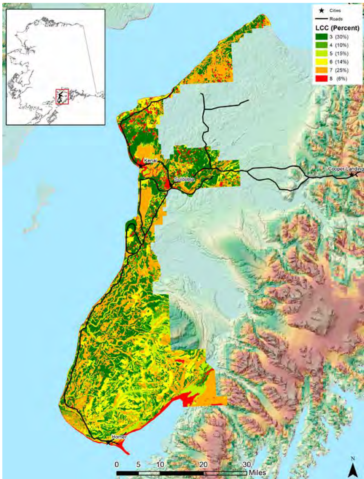
Figure A.4—Western Kenai Peninsula land capability class (USDA NRCS 2019b).
