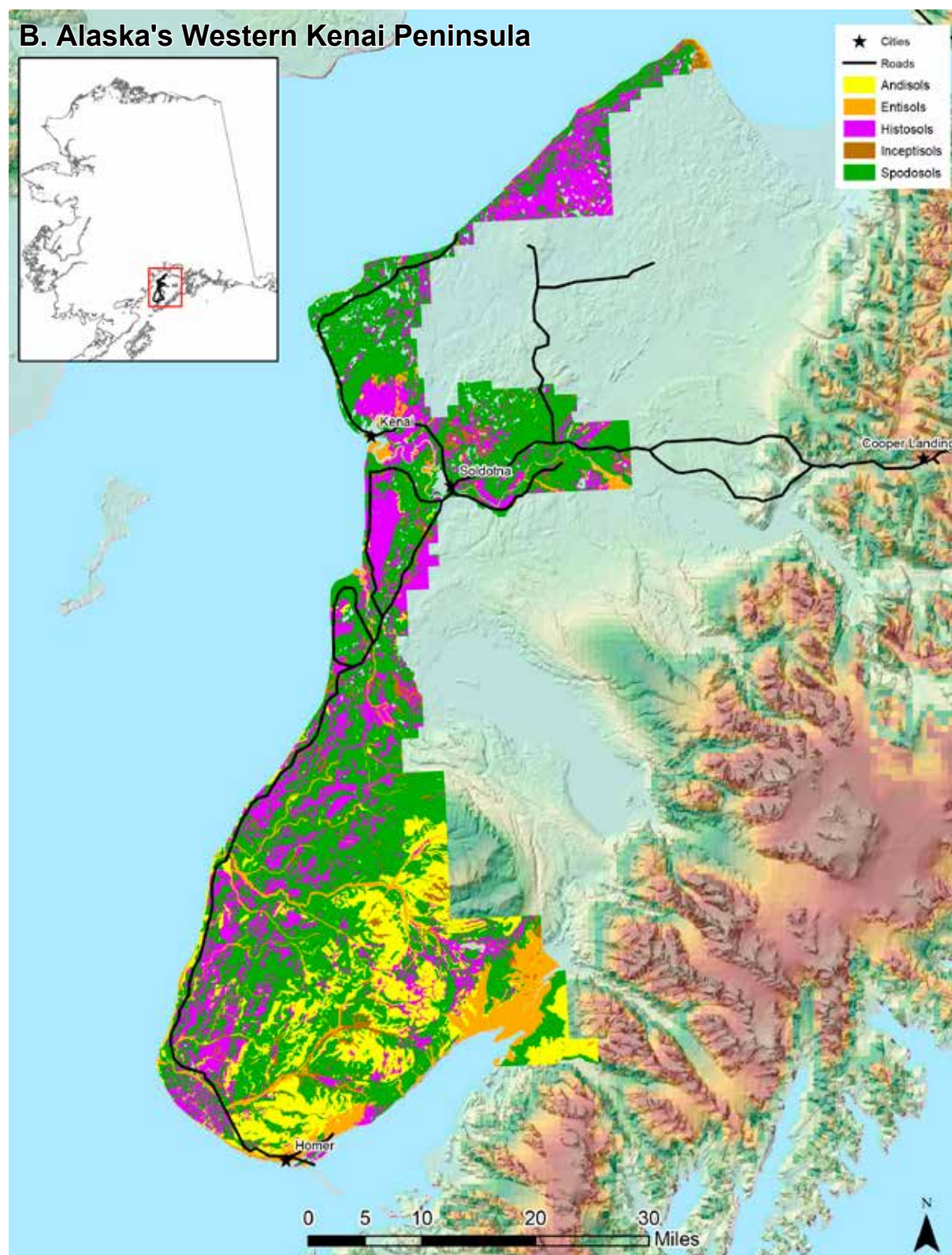
Figure 1.6 (continued)—Soil taxonomy orders (Andisols = yellow, Entisols = orange, Histosols = purple, Inceptisols = brown, and Spodosols = green) in the (A) Matanuska-Susitna Valley survey areas (USDA NRCS2019a) and (B) western part of the Kenai Peninsula (USDA NRCS 2019b)
