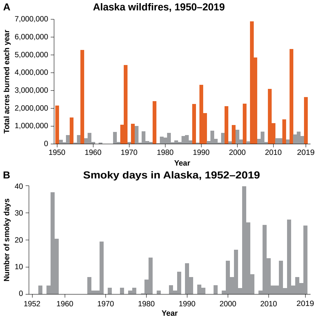
Figure 1.2—(A) Comparing total acres burned each year since 1950, there have been more years with more than 1 million ac (404 686 ha) burned (orange bars) in the most recent decades. Total acres burned each year are expected to increase with climate change. (B) The number of smoky days due to wildfire, with visibility restricted by smoke, has increased over the past two decades.
