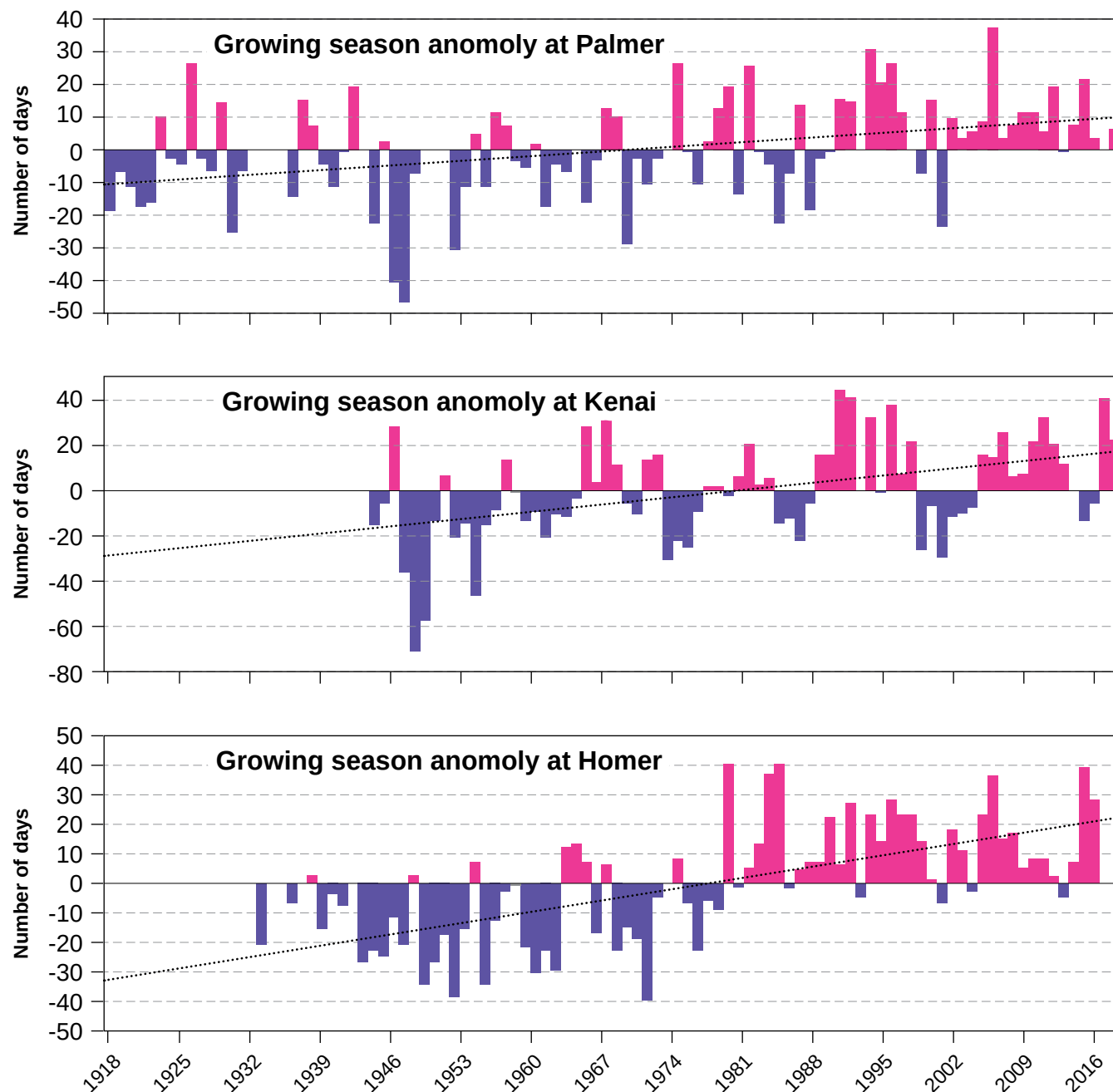
Figure 5.1—Growing season differences (anomaly or deviation) from the long-term average for Homer, Kenai, and Palmer weather stations from 1918 to 2017. Data availability at each weather station varied, but long-term mean temperatures include all available data at each weather station (Palmer: 1918–2017, Kenai: 1944–2017, Homer: 1933–2017). The take-home message is that each location has more growing days since the 1980s.
