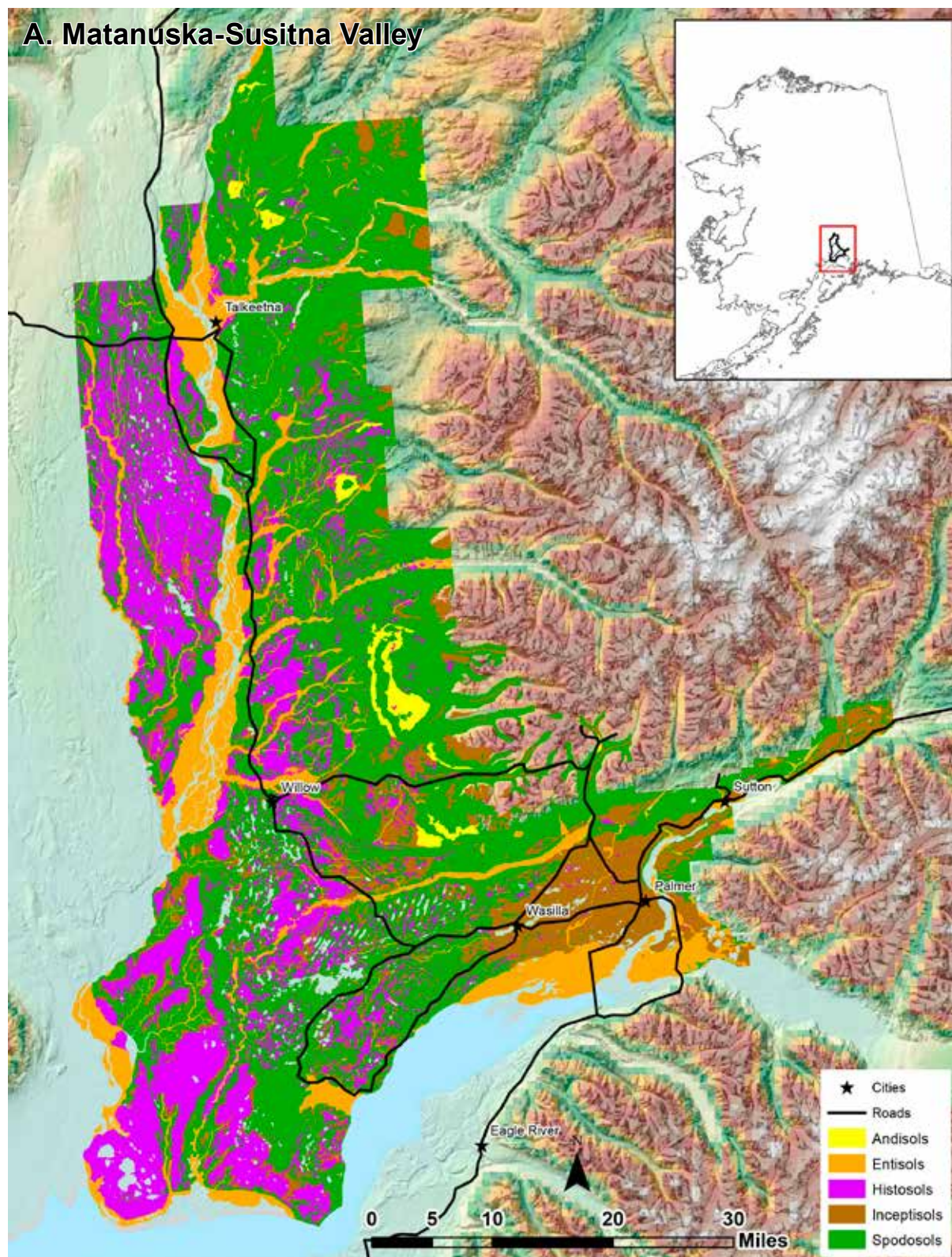
Figure 1.6—Soil taxonomy orders (Andisols = yellow, Entisols = orange, Histosols = purple, Inceptisols = brown, and Spodosols = green) in the (A) Matanuska-Susitna Valley survey areas (USDA NRCS 2019a) and (B) western part of the Kenai Peninsula (USDA NRCS 2019b)
