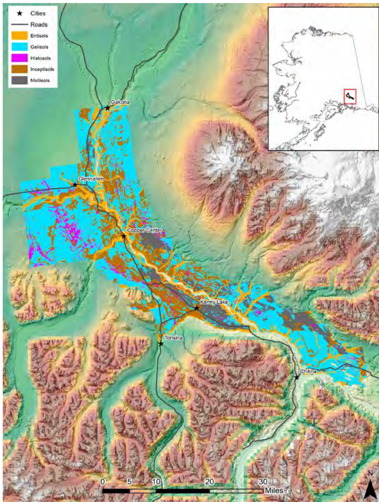
Figure A.9—Copper River area soil taxonomy order (USDA NRCS 2019c).
