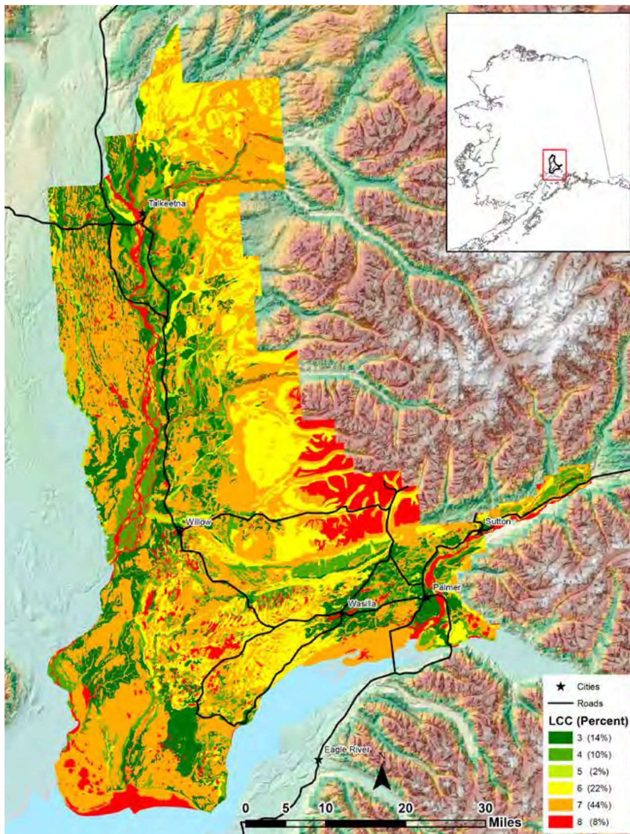
Figure A.3—Matanuska-Susitna Valley land capability class (USDA NRCS 2019a).
