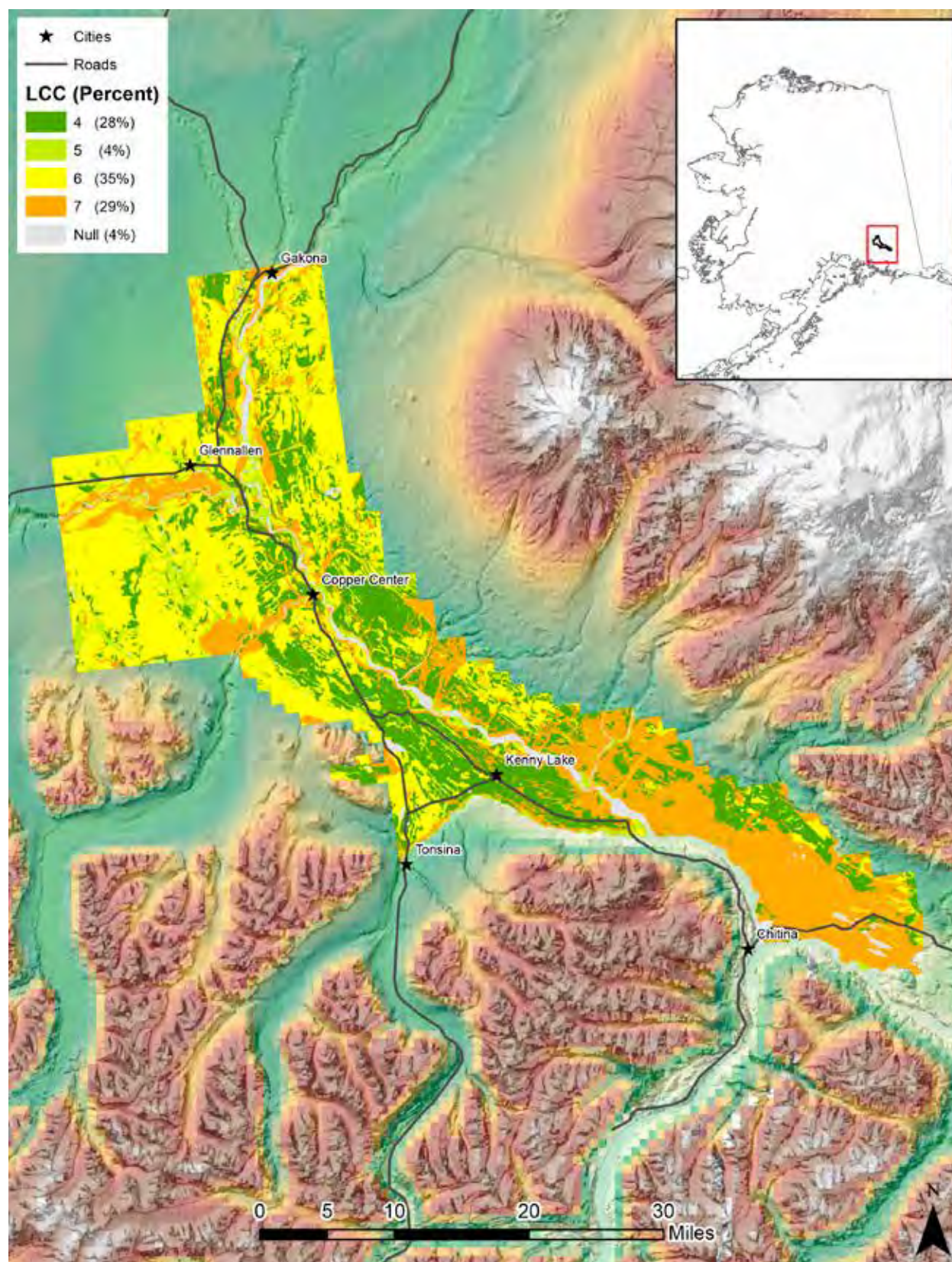
Figure A.10—Copper River soil survey area land capability class (USDA NRCS 2019c).
