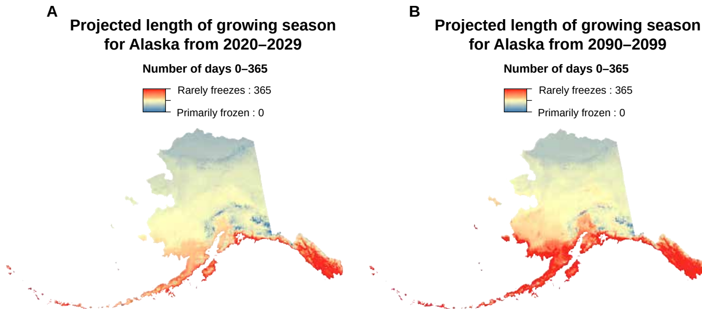
Figure 1.3—Growing season is the time of year that is favorable for plant growth. Climate projections from downscaled, Coupled Model Intercomparison Project Five (CMIP5) five-model show the mean length of growing season (numbers of days: 0–365) at 771 by 771 m spatial resolution and representative concentration pathway (RCP) 8.5, a high-end emissions scenario that aligns with increasing current greenhouse gas emissions for (A) 2020–2029 and (B) 2090–2099. Note that a longer growing season, indicated by red colors, is expected to expand northward with notable change across the southern half of the state. The least amount of change is expected in northern Alaska. Data from the Alaska Center for Climate and Policy.
