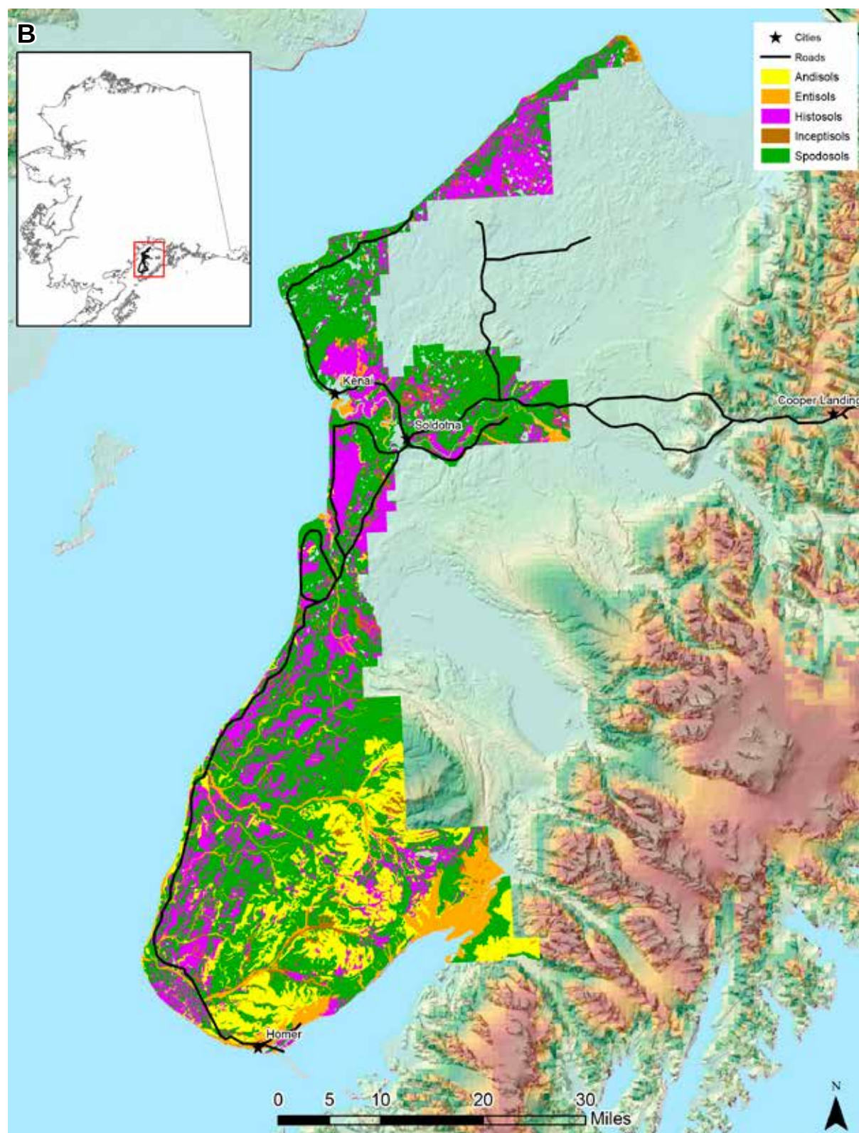
Figure A.2 (continued)—Soil taxonomy order in the (A) Matanuska-Susitna Valley area and (B) western Kenai Peninsula survey areas (USDA NRCS 2019a, 2019b.).
