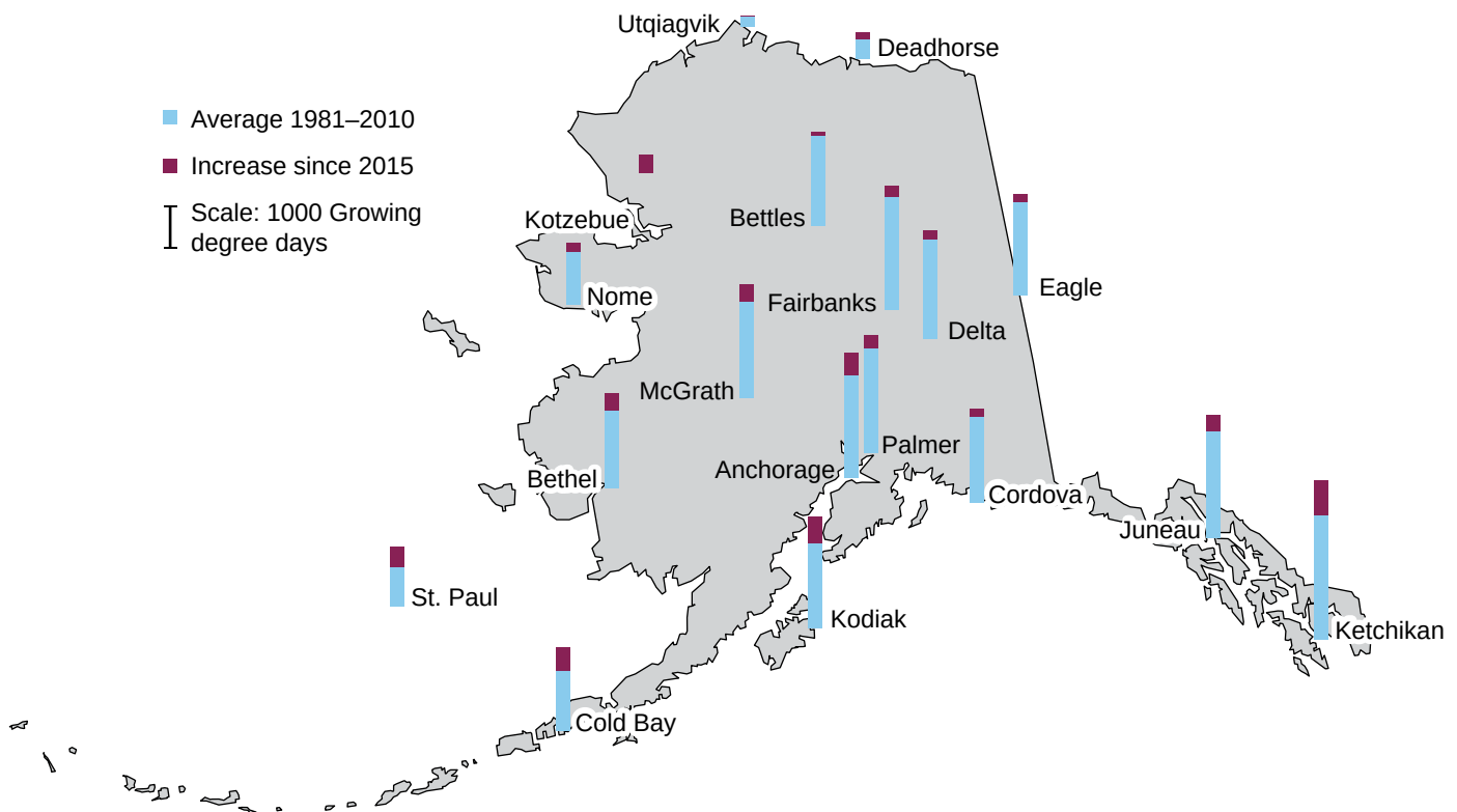
Figure 1.5—Growing degree days for a 40 °F (4.4 °C) crop for different communities in Alaska, with blue bars noting the average growing degree days from 1981 to 2010 and the red portion of the bar noting the increase in growing degree days since 2015 through 2018 in comparison to the average. Adapted from Nancy Fresco, Scenarios Network for Alaska+ Arctic Planning and Rick Thoman, Alaska Center for Climate Assessment and Policy. Data source: NOM/NCEI, NDAWN, Canadian Journal of Plant Science, 2006.
