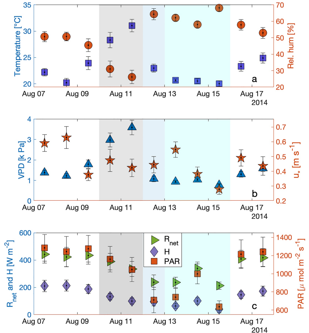
Figure 1. Environmental conditions during the 10 day period that includes the smoke event (shaded in gray). On 12 August the site experienced widespread overcast conditions and rain (shaded in blue). Cloud cover persisted between 13 and 15 August (shaded in cyan). Error bars indicate the standard error around the mean for each quantity.
