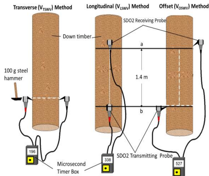
Figure 1. Measuring pattern using the FAKOPP acoustic tool; white dash lines indicate measured probe distance.
