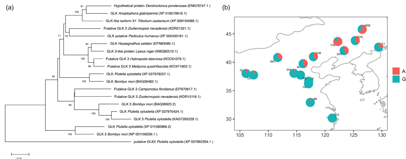
FIGURE 6 Exploring the potential functional relevance of a missense mutation under positive selection ( F_{ST} = 0.335 ) within the Anoplophora glabripennis glycerol kinase gene AGLA000593 . (a) Phylogenetic tree of several glycerol kinase proteins from different insect species, including A. glabripennis . All NCBI accessions are provided. The neighbor-joining tree was done in MEGAX (with 1000 bootstraps). Only the branch supports above 70% are indicated. The closest homology for the ALB protein was found with D. ponderosae . (b) Geographic map of the allele frequency distribution for the glycerol kinase gene AGLA000593 across the 16 Chinese ALB populations studied by GBS technology. G refers to the reference allele and A to the alternative allele (the missense mutation)
