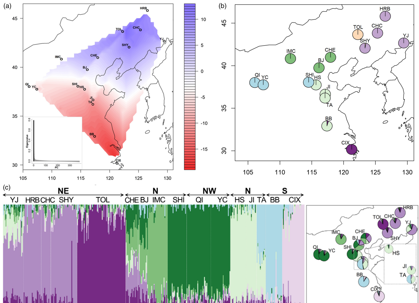
FIGURE 3 (a) Interpolated gradient map of the spatial genetic structure of the Asian longhorned beetle based on the first positive eigenvalue of spatial principal component analysis (sPCA). Eigenvalues of sPCA are displayed on the inset. Positive eigenvalues correspond to global genetic structure, and negative eigenvalues indicate local genetic structure. The color ramp shows values for lagged scores. (b) DAPC analysis using SNPs of 16 sampled ALB populations in China. Map with the 16 populations color-coded as per the DAPC population clustering results. (c) Bar plot and interpolated map of ancestry coefficients across 16 populations ( k = 7 ). A total of 6102 SNPs were used in the analysis. Each color-coded pie represents one of the 16 sampled ALB populations in China. Population codes are explained in Table 1. A total of 6102 SNPs were used
