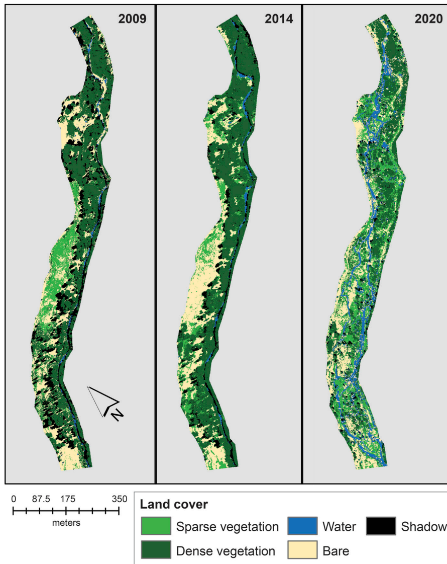
FIGURE 10 | Isocluster unsupervised classification of surface vegetation at Whychus Canyon Preserve Phase 1 site using National Agricultural Imagery Program NDVI datasets. Restoration occurred at this site in 2016.
