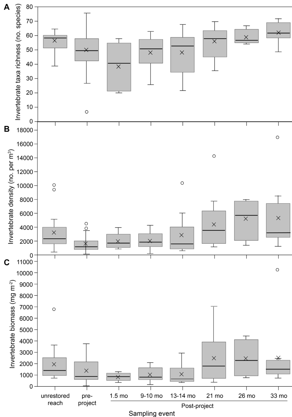
FIGURE 8 | South Fork McKenzie River benthic macroinvertebrates from reference (unrestored) habitats, pre-restoration, and in the months post-restoration for: (A) invertebrate taxa richness; (B) invertebrate density; and (C) invertebrate biomass. Boxplot center line is the median, and X is the data mean.
