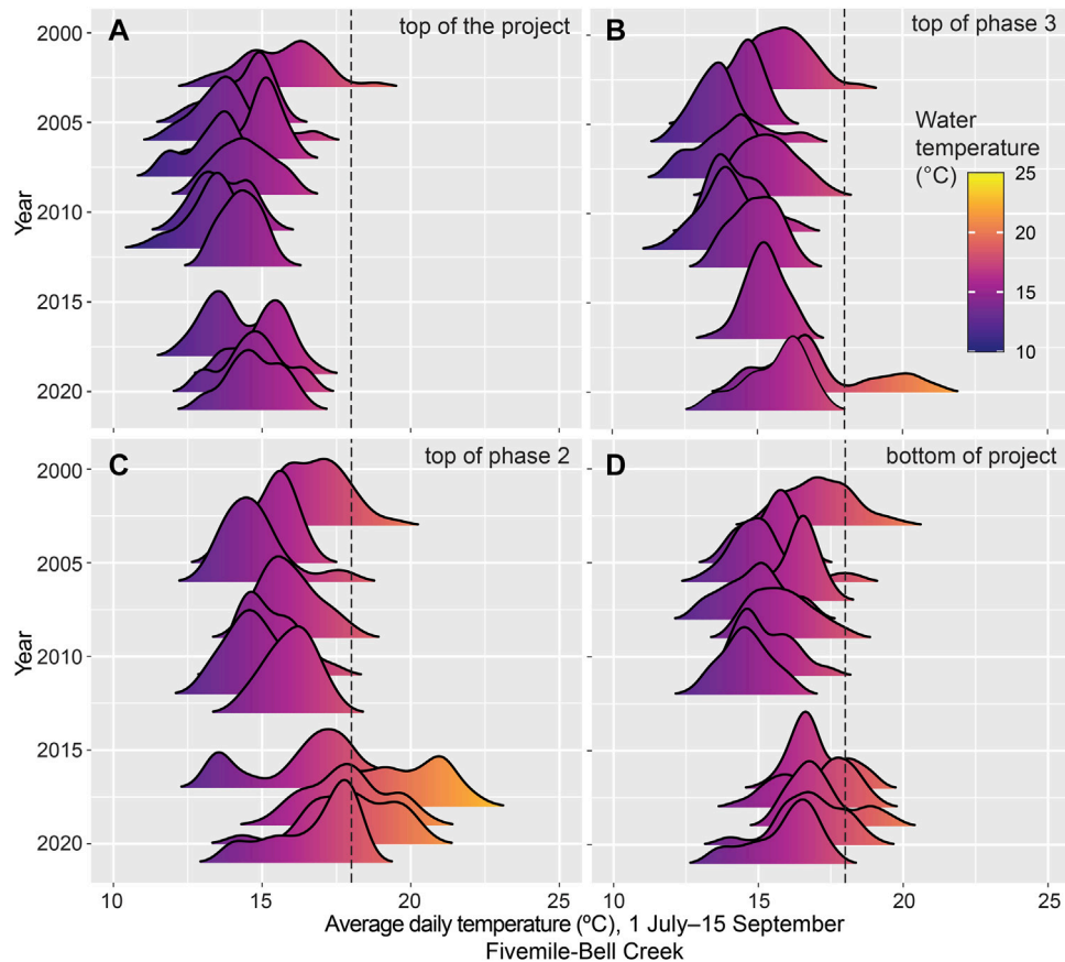
FIGURE 6 | Stream temperature over time at Fivemile Bell site that drains into Tahkenitch Lake on the south coast of Oregon, United States.
