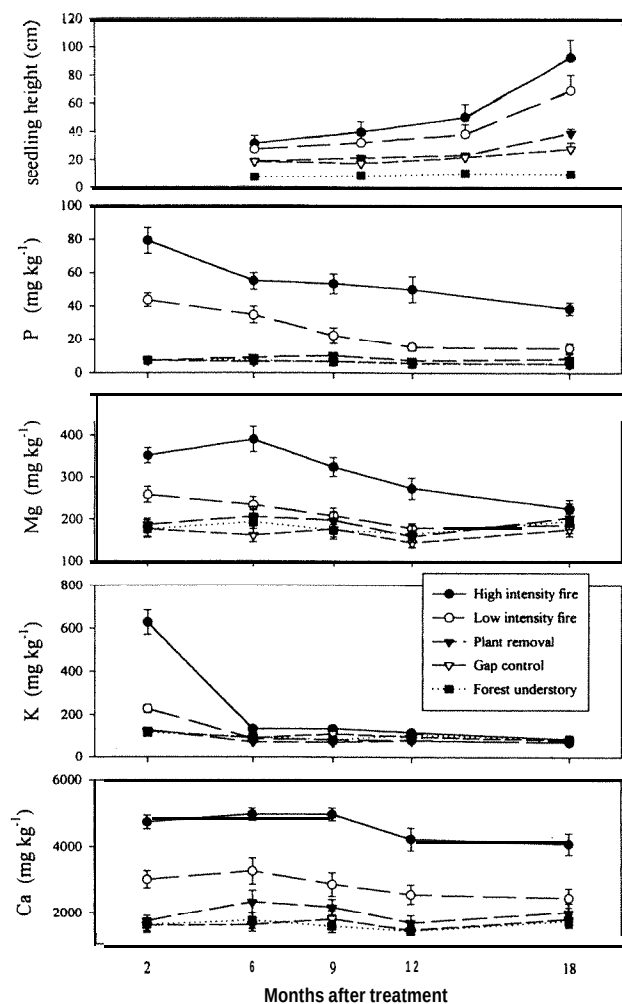
Figure 1. Seedling heights of Anadenanthera colubrina , and Mehlich-I extractable soil concentrations of P, Mg, Ca, and K in soil samples (0–8 cm depth) in four treatments and understory forest sites at five sampling times over an 18-month period following fires (bars = S.E., n=16 ).
