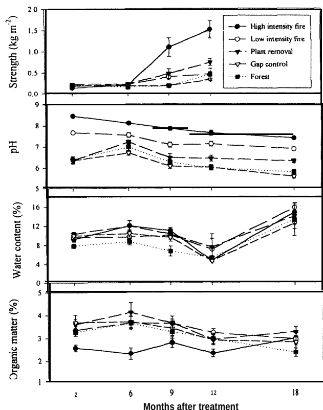
Figure 3. Soil pH, air-dry water content, and organic matter content measured in soil (0–8 cm depth) in the four treatments and understory forest sites at five sampling times over an 18-month period following burns. Soil strength was measured at the soil surface with a soil penetrometer at four sampling periods over a 12-month period following burns. Water content is expressed as percent of air-dry weight (bars = SE., n=16 ).
