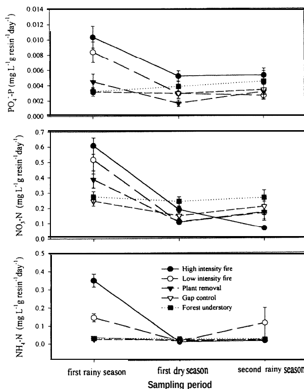
Figure 2. Resin-available ammonium, nitrate, and phosphate in four treatments and understory forest sites determined from exchange resins buried in soil at 5 cm depth during three periods following fires (bars = S.E., n=16 ). Resins were buried for approximately 3 months during each period. Time since fires of sampling periods were: first rainy season (2–5 months), first dry season (8–11 months), and second rainy season (15–18 months).
