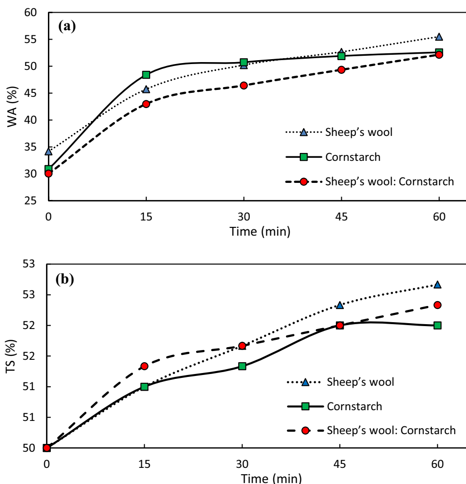
Fig. 12 Measurements over time. a Water absorption (WA) and b thickness swelling (TS) measurements taken from each of our three binders (sheep's wool, cornstarch, and sheep's wool:cornstarch) at 15-min intervals for 1 h
