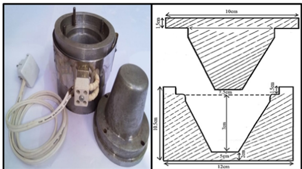
Fig. 2 CK60 steel mold designed for the study. CAD design of the mold used to produce biodegradable pot samples
