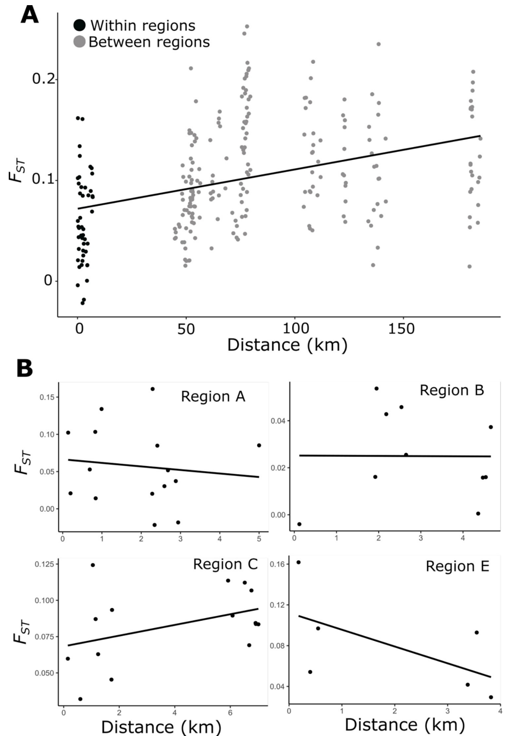
Fig 4. Isolation by distance plots. Segregation of allele frequencies (measured by F_{ST} ) is shown between pairs of sites versus geographic distance. A. All site pairs in this study, with comparisons within regions shown in black and comparisons between regions in grey. B. Within-region site comparisons, grouped by region (region D is omitted since only two sites were sampled).
