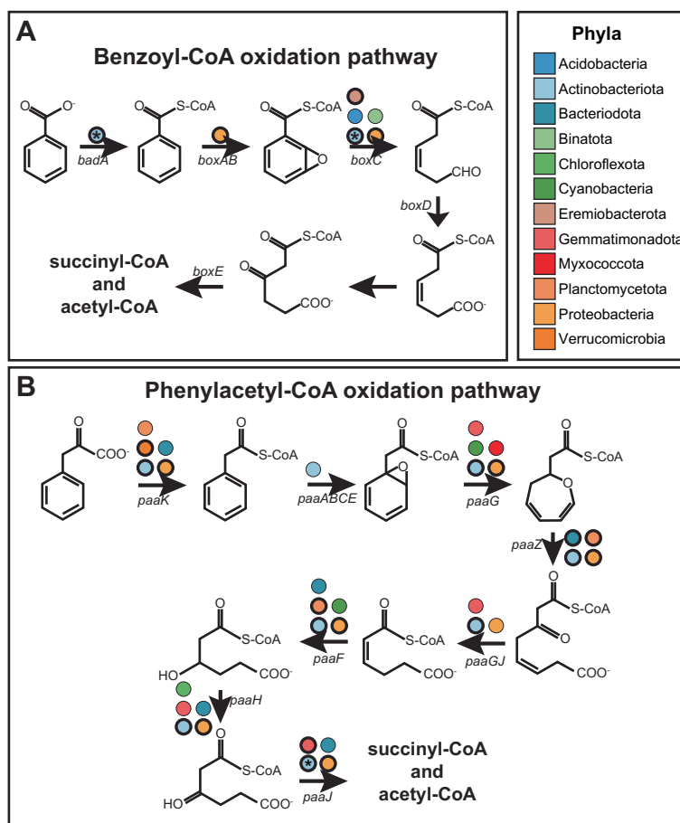
Extended Data Fig. 7 | Genomic evidence of other aerobic aromatic C degradation pathways. The benzoyl-CoA oxidation pathway ( a ) and phenylacetyl-CoA oxidation pathway ( b ) with overlaid gene names and whether there was encoded or expressed evidence of these genes. Colored circles indicate whether a MAG from that phyla encoded that gene, bolded circles indicate that metatranscriptomic reads mapped to the gene, and asterisks indicate the gene was being highly expressed in any given condition.
