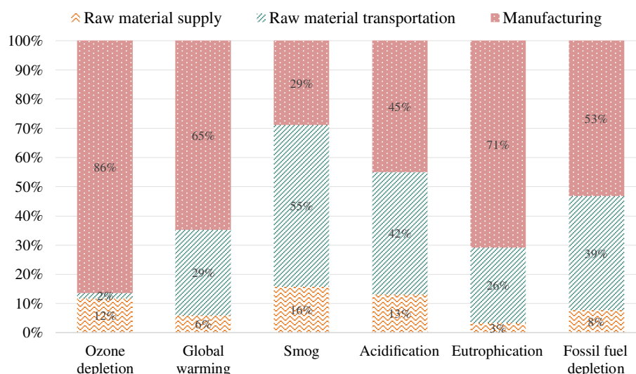
Figure 2. Contribution of the life-cycle stages of pallet repair and remanufacturing to the resulting environmental impact.
