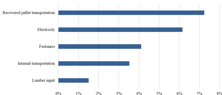
Figure 3. Sensitivity of parameters on global warming impact of pallet repair/remanufacturing (declared unit: one repaired/remanufactured pallet), mass allocation.
