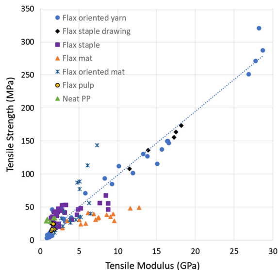
Fig. 10 Tensile strength versus tensile modulus of flax fiber reinforced polypropylene composites with flax fibers in the forms of pulp, staple fibers, mats, and yarns, random or oriented (Heijenrath and Peijs 1996; Oksman 2000; Van den Oever et al. 2000; Cantero et al. 2003; Madsen and Lilholt 2003; Arbelaiz et al. 2005a, b; Miao and Shan 2011; Kannan et al. 2013; Derbali et al. 2016; Wu et al. 2016; Bar et al. 2018, 2019)
