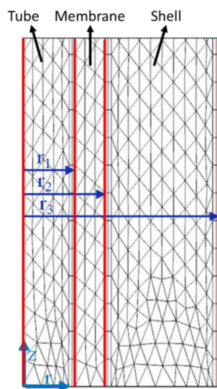
Figure 3. Schematic of a segment of the half longitudinal section of a single fiber mesh distribution.
