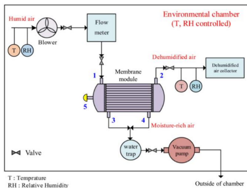
Figure 1. Schematic of a lab-scale membrane air dehumidification system. Reproduced with permission from Reference [7]. Copyright 2021 Wood and fiber Science.
