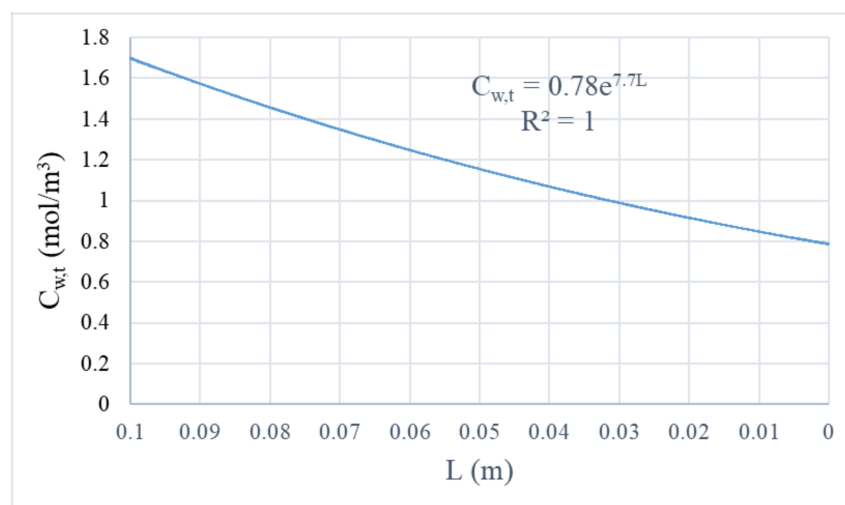
Figure 5. Axial concentration distribution of water vapor in the tube domain of hollow fiber membrane (air velocity = 0.028 m/s, initial concentration of water vapor = 1.72 \text{ mol/m}^3 , and vacuum pressure = 67.7 kPa).
