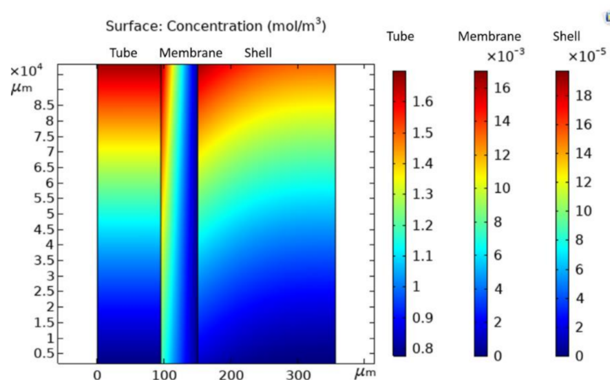
Figure 4. Distribution of concentration of water vapor in three domains of a hollow fiber membrane (air velocity = 0.037 m/s, initial concentration of water vapor = 1.72 \text{ mol/m}^3 , and vacuum pressure = 77.9 kPa).
