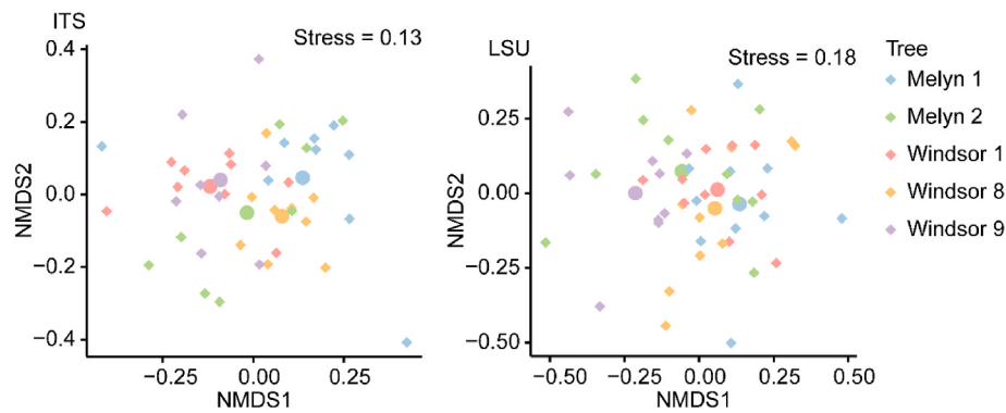
Fig. 5. NMDS ordinations of fungal communities for samples (n = 65) taken from five trees (n = 13 drill holes per tree), according to ITS and LSU barcodes. Plots are based on Raup-Crick distance matrices, k = 3, dimensions 1 and 2 are displayed. Individual points are coloured by tree, whilst the larger points represent centroids for each.
