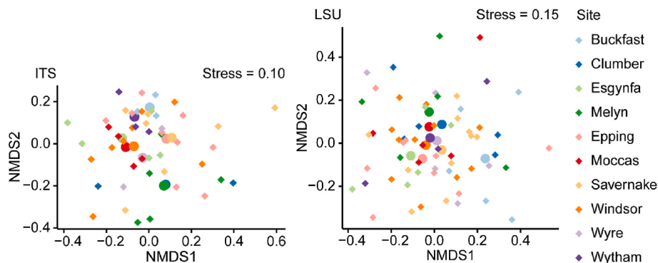
Fig. 4. NMDS ordinations of fungal communities for all trees sampled once at breast height (n = 66), according to ITS and LSU barcodes. Plots are based on Raup-Crick distance matrices, k = 3, dimensions 1 and 2 are displayed. Individual points are coloured by site, whilst the larger points represent centroids for each.
