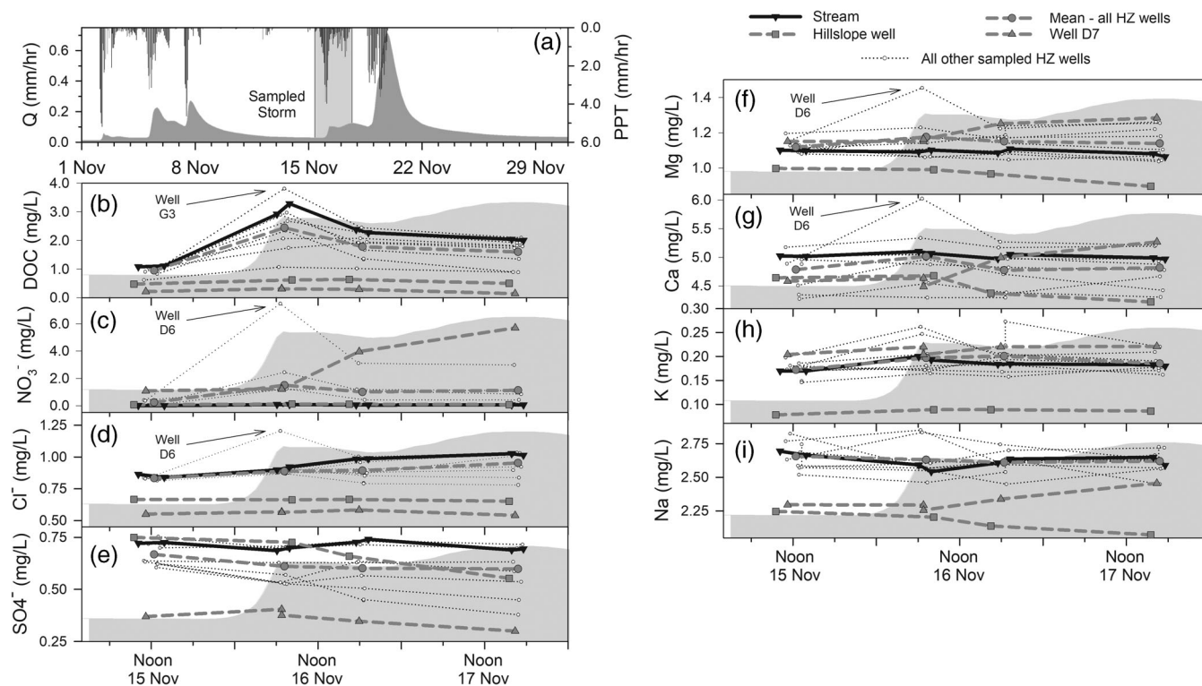
FIGURE 2 (a) Hourly precipitation from PRIMET benchmark station (black bars; Daly & McKee, 2019) and hourly mean discharge recorded at the WS1 gage (dark grey shading; Johnson et al., 2020). Shaded rectangle, spanning 15–17 November indicates the storm during which samples were collected. (b–i) Solute concentrations measured in the stream and the well network during the storm (Wondzell & Corson-Rikert, 2016)
