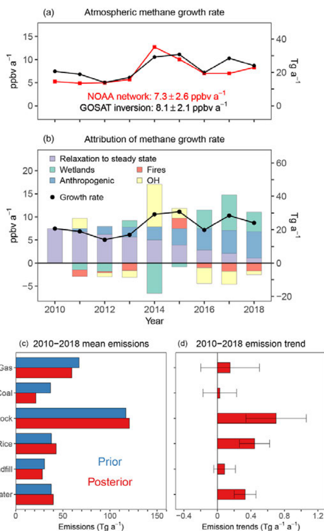
Figure 11. Attribution of the 2010–2018 trend in atmospheric methane by inversion of GOSAT satellite observations. The top panel shows the growth rates of atmospheric methane for individual years as measured by the NOAA surface network and as inferred from the inversion of GOSAT observations, indicating good agreement between the two and an acceleration of the methane trend after 2013. The middle panel shows the attribution of the trend to different sources and to the methane sink (OH), highlighting major contributions from anthropogenic sources and from wetlands. The bottom panels show the major anthropogenic emissions and their trends by sectors, indicating a major contribution of livestock to the methane trend. Adapted from Zhang et al (2021).
