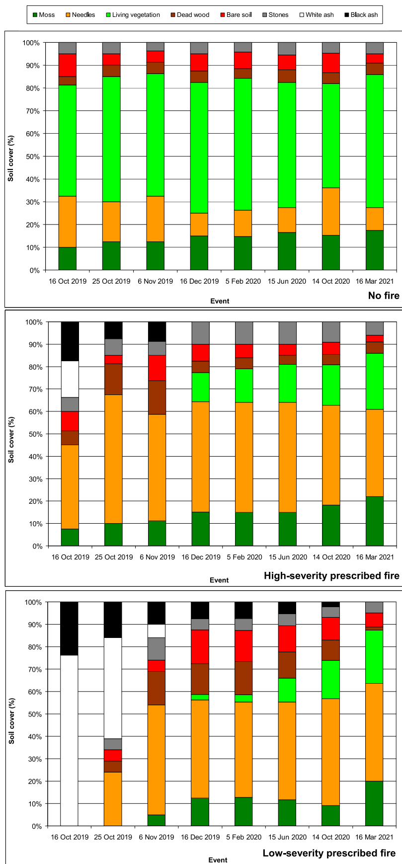
Fig. 3. Evolution of the soil covers in plots under three soil conditions (no fire (a), high-severity prescribed fire (b) and low-severity prescribed fire (c)) after the prescribed fire and eight subsequent precipitation events (excluding the first rainfall) in La Moraleja forest (Castilla La Mancha, Spain).
