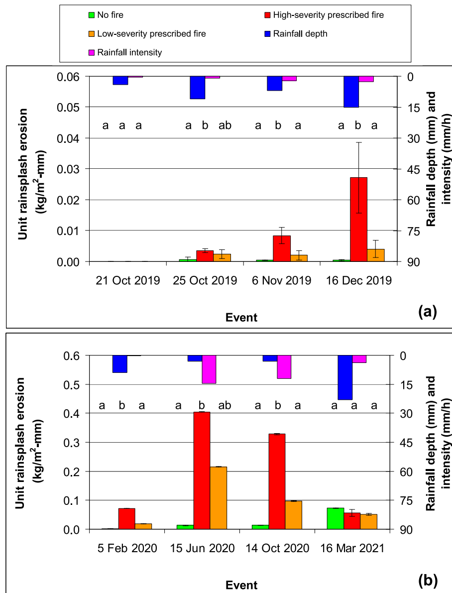
Fig. 2. Unit rainsplash erosion measured at the plot scale under three soil conditions (no fire, high-severity prescribed fire and low-severity prescribed fire) after eight precipitation events in La Moraleja forest (Castilla La Mancha, Spain). (a) Soil losses for the period 21 Oct 2019–16 Dec 2019. (b) Soil losses for the period 5 Feb 2020–16 Mar 2021. Different letters indicate significantly different mean unit rainsplash erosion rates among the soil conditions.
