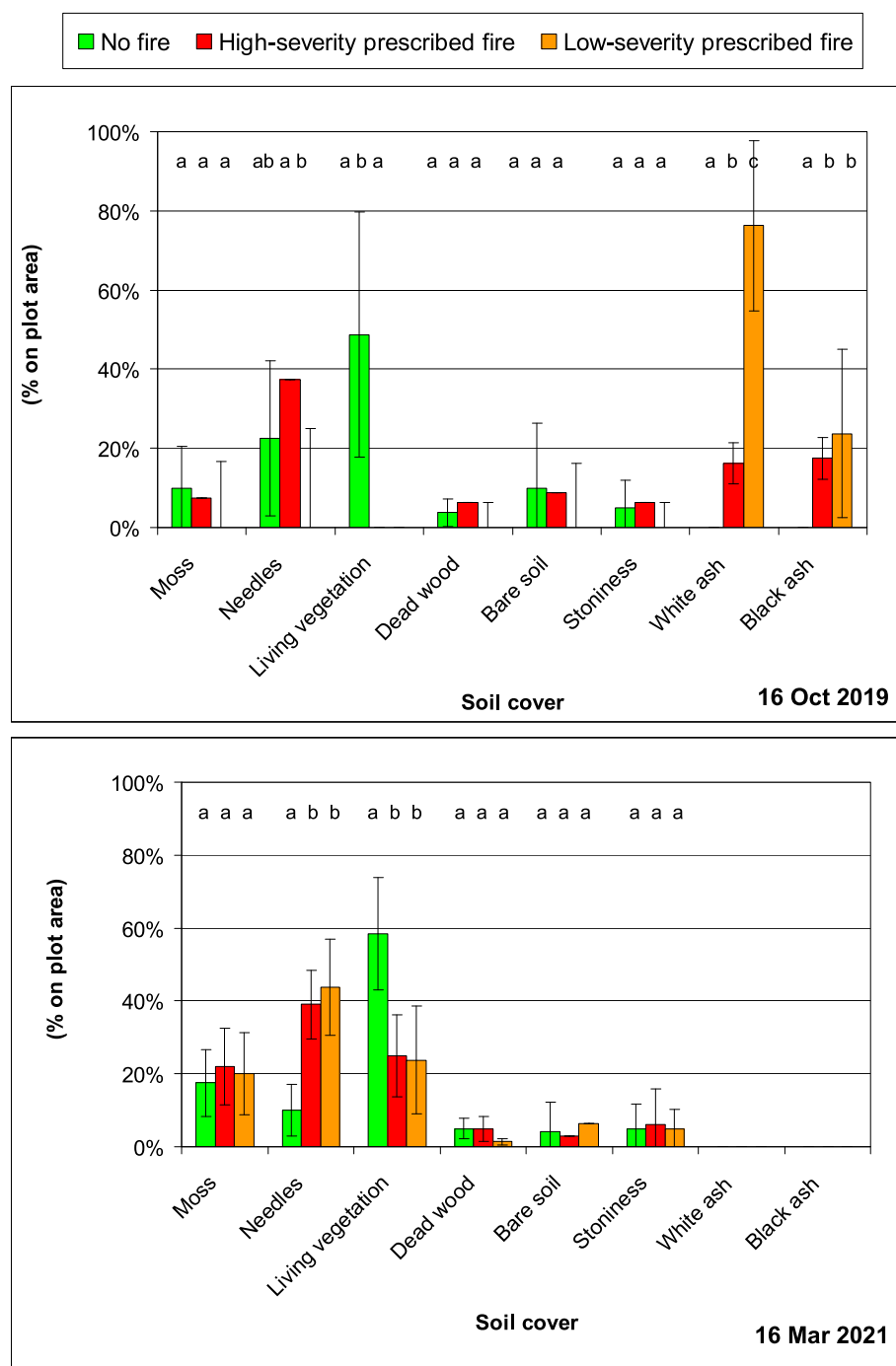
Fig. 4. Soil covers surveyed at two dates in plots under three soil conditions (no fire, high-severity prescribed fire and low-severity prescribed fire) (immediately after fire (upper panel) and one and a half years after the fire (lower panel)) in La Moraleja forest (Castilla La Mancha, Spain). Different letters indicate significantly different cover among the soil conditions.
