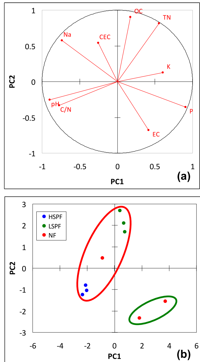
Fig. 6. Loadings of the original variables (a, physico-chemical properties of soil), and scores with relevant clusters (b) on the first two Principal Components (PC1 and PC2) provided by the Principal Component Analysis coupled by Analytical Hierarchical Cluster Analysis applied to soil samples under three soil conditions (no fire, NF; high-severity prescribed fire, HSF; low-severity prescribed fire, LSF) in the study area (La Moraleja forest, Castilla La Mancha, Spain). Notes: EC = electrical conductivity; OC = organic carbon; TN = total nitrogen; C/N = carbon to nitrogen ratio; P = phosphorous; K^+ = potassium; Na^+ = sodium; CEC = cation exchange capacity.
