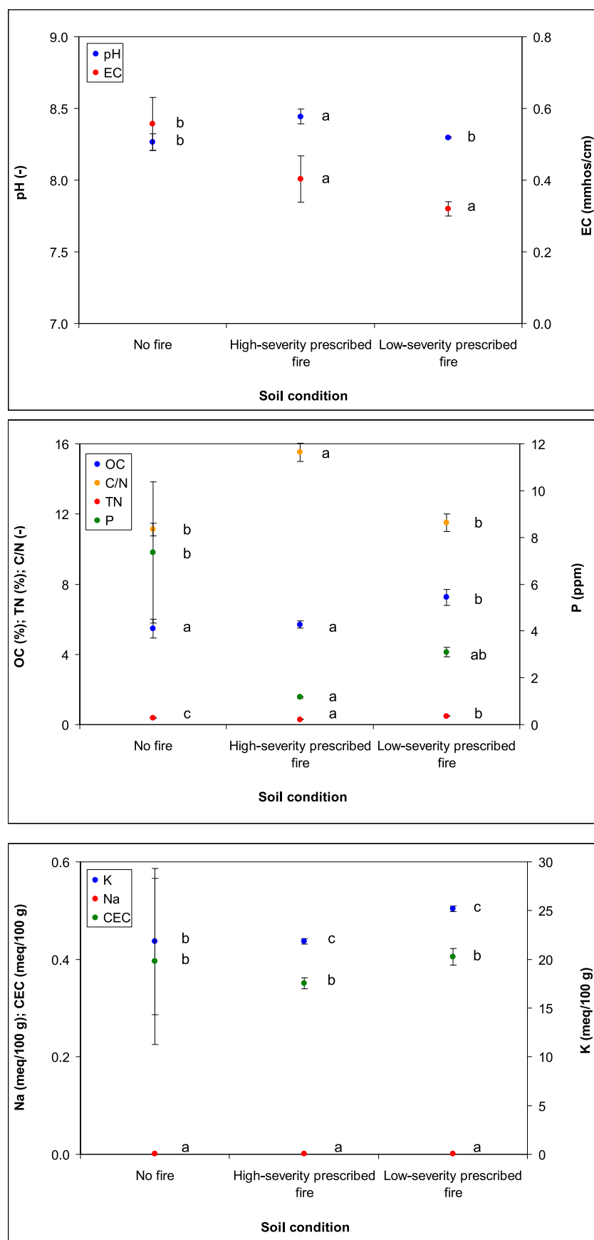
Fig. 5. Main physico-chemical properties of soils under three conditions (no fire, high-severity prescribed fire, and low-severity prescribed fire) immediately after burning (16 October 2019) in La Moraleja forest (Castilla La Mancha, Spain): pH and electrical conductivity (EC) (a); organic carbon (OC), carbon/nitrogen (C/N) ratio, total nitrogen (TN), and phosphorous (P) (b); and potassium ( K^+ ), sodium ( Na^+ ), and cation exchange capacity (CEC) (c). Different letters indicate significantly different properties among the soil conditions.
