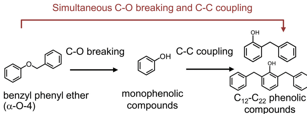
Scheme 1 Transformation pathways for benzyl phenyl ether (α-O-4) into C 12 –C 22 phenolic compounds.
