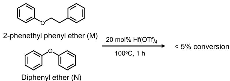
Fig. 2 Conversion of 2-phenethyl phenyl ether and diphenyl ether by \text{Hf(OTf)}_4 . Reaction conditions: feed = 0.26 mmol 2-phenethyl phenyl ether or diphenyl ether, feed/heptane/dodecane (internal standard) = 1.0 : 8.5 : 0.5 by weight, \text{Hf(OTf)}_4 = 20 mol%, 100 °C, 1 bar, 1 h.
