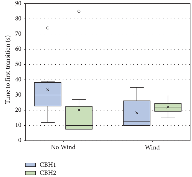
FIGURE 3: Time to first sustained surface-crown transition for nonwind-driven and wind-driven fires at the two examined crown base heights, where CBH1 = 60 cm and CBH2 = 70 cm; the symbols outside of the box plots for the nonwind cases are outliers.
