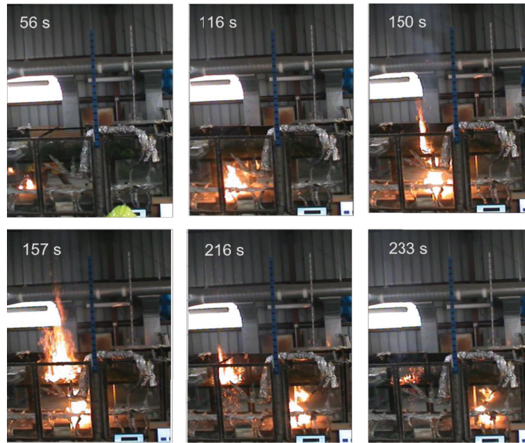
FIGURE 8: Special case of marginal spread at CBH = 0.7 m and no wind. The progression of images extracted from the experiment video shows the transition location, the development of the crown flame, and the eventual natural extinguishing of the flame which leaves a considerable portion of the fuel bed unburned.
