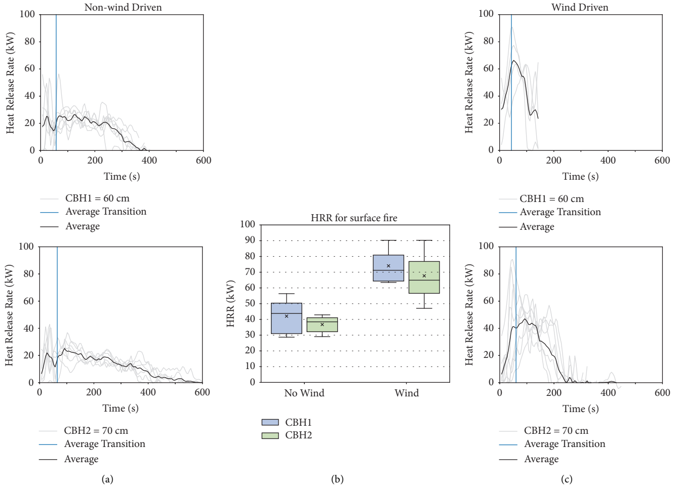
FIGURE 5: Surface fire heat release rate in nonwind-driven fires (a), wind-driven fires (c), and the box and whisker plot with average heat release rate for all experiments (b). For the box plot, the cross represents the mean, the horizontal bar represents the median, the bottom of the box represents the 25th percentile, the top of the box represents the 75th percentile, the bottom of the whisker is the minimum data point, and the top of the whisker is the maximum data point.
