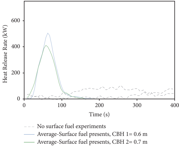
FIGURE 9: Crown fire behavior of wind-driven experiments conducted with a surface fuel bed (solid lines) and without a surface fuel bed (dashed lines).
