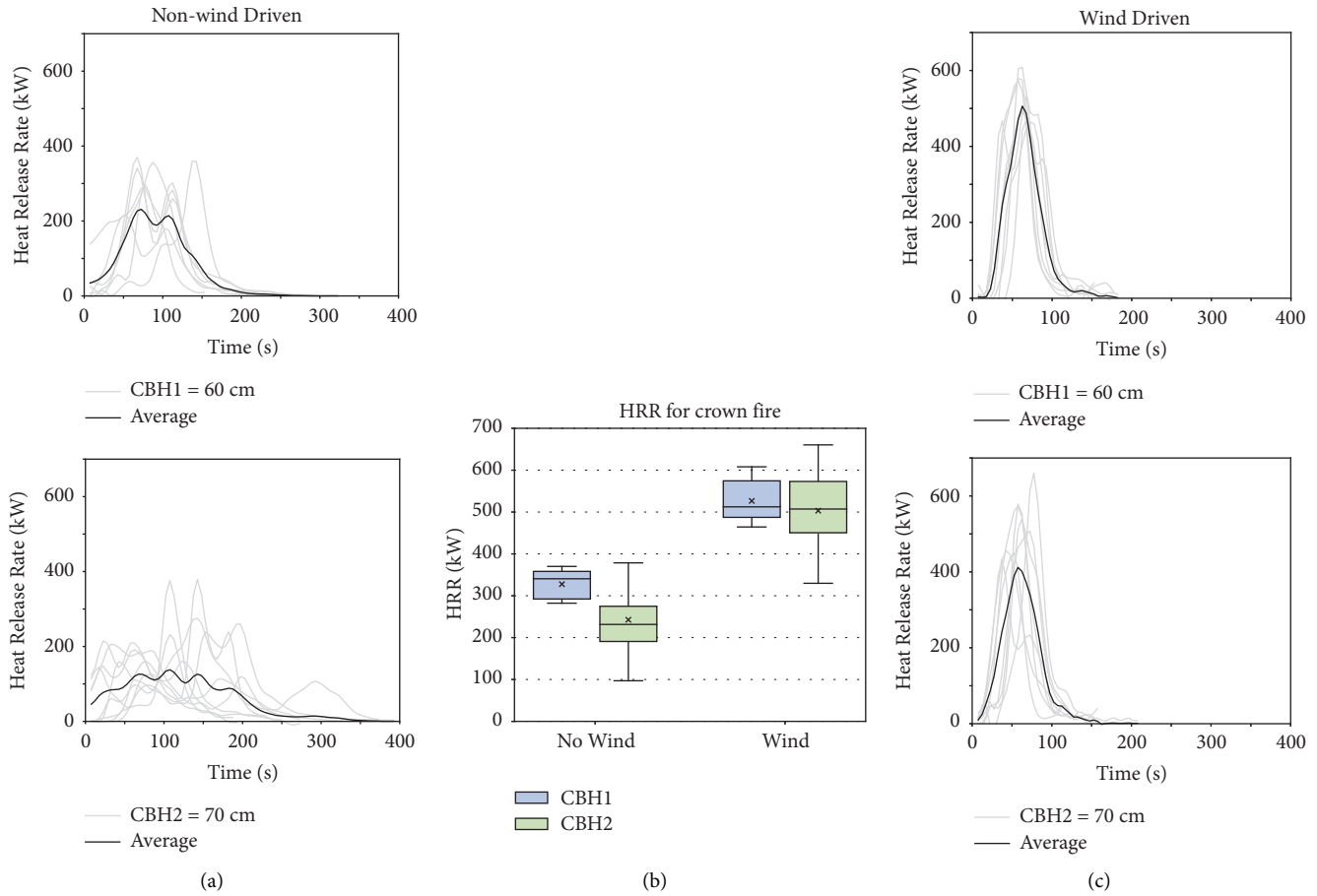
FIGURE 4: Crown fire heat release rate in nonwind-driven fires (a), wind-driven fires (c), and the box and whisker plot with average heat release rate for all experiments (b). For the box plot, the cross represents the mean, the horizontal bar represents the median, the bottom of the box represents the 25th percentile, the top of the box represents the 75th percentile, the bottom of the whisker is the minimum data point, and the top of the whisker is the maximum data point.
