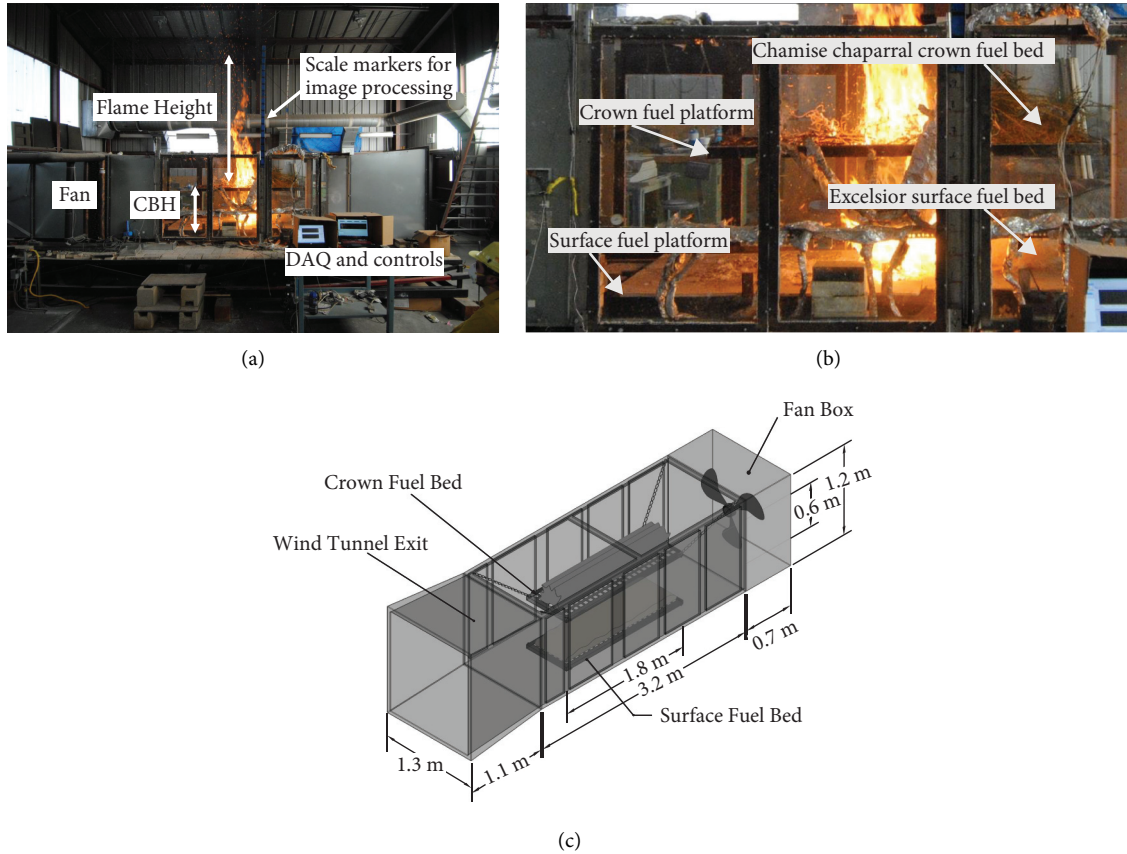
FIGURE 1: Experimental setup for wind tunnel experiments, from top to bottom: (a) complete experimental setup showing the location of the wind tunnel fan, data acquisition system (DAQ) and controls, crown base height (CBH) distance, flame height, and metal bar with markers used as a scale during image processing, (b) a close-up view of the test section showing the location of the crown fuel bed platform, chamise chaparral fuels, surface fuel bed platform, and excelsior surface fuels, and (c) schematic with part labels and dimensions.
