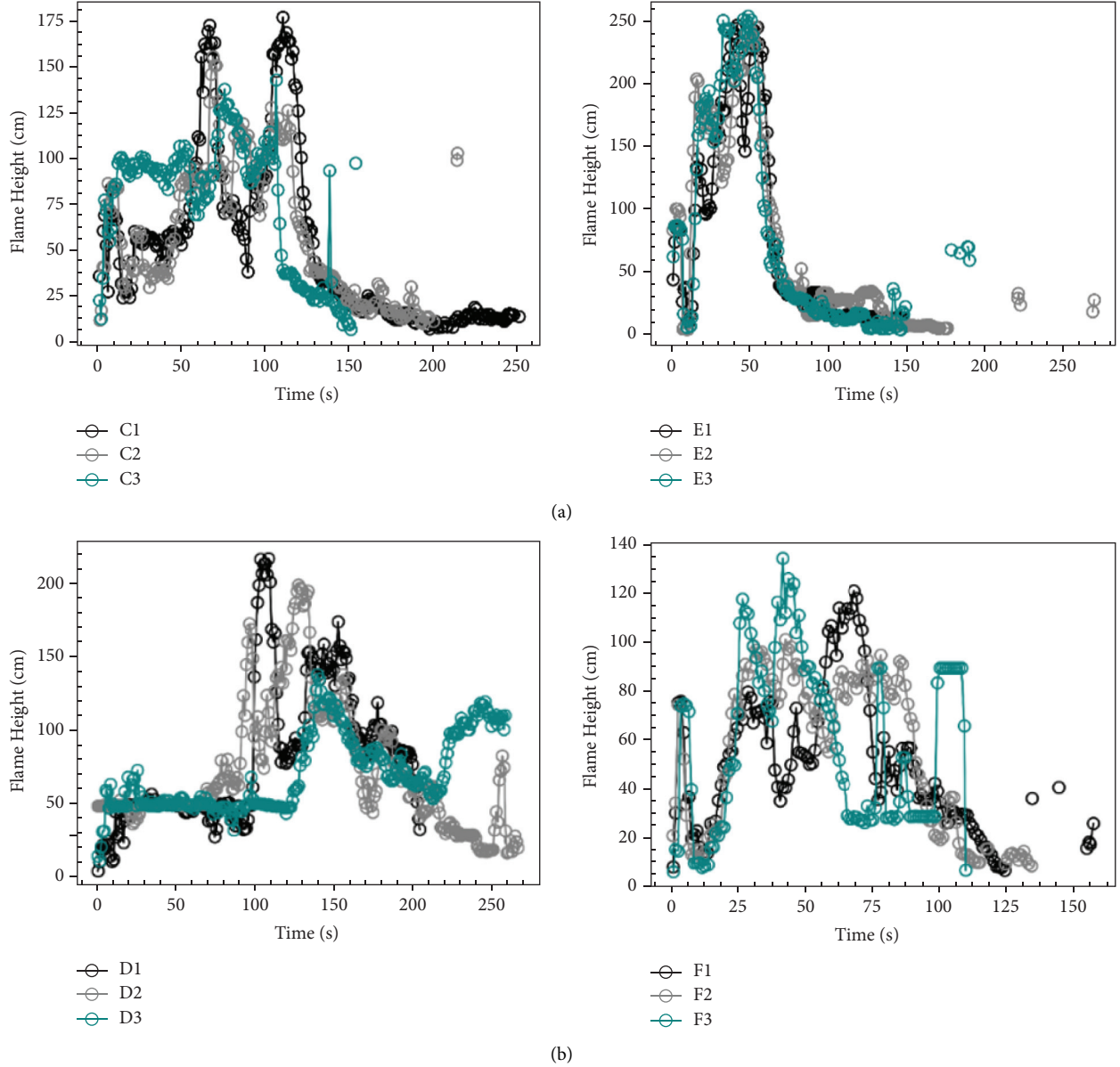
FIGURE 7: Time evolution of crown flame height in experiments with CBH = 0.7 m under wind conditions. (a) No wind. (b) \bar{U} = 1 m/s. Initial time, t = 0 , is set as the time at the transition to the crown layer for each experiment. Experiments C1 and F3 are representative experiments for each experimental configuration.
