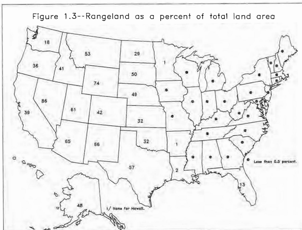
Figure 3.—Rangeland as a percent of total land area by State.
