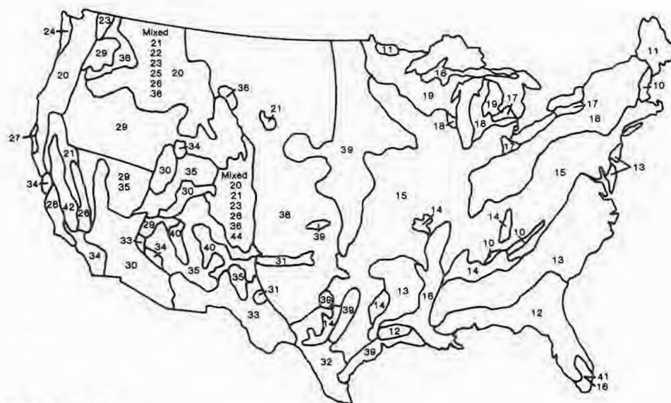
Figure 5.—Forest and range environmental system (FRES) ecosystems of the United States.
