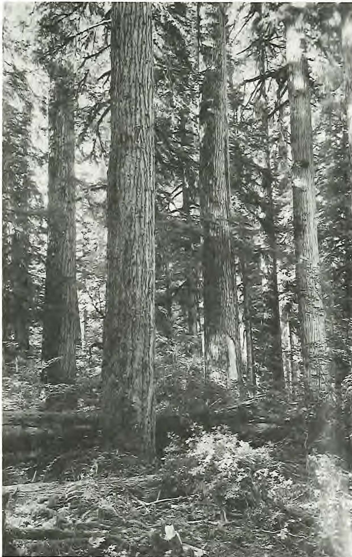
Figure 20.—By far the greatest change in Pacific Coast forests has been the reduction in area of old growth.
