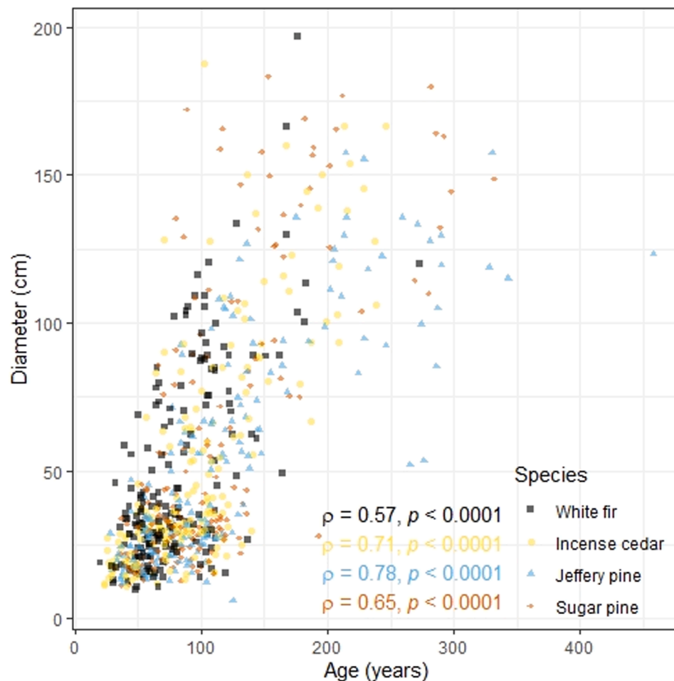
Fig. 2. Relationship between diameter and ring count (age) by species for sampled trees. Spearman correlation coefficients ( \rho ) and associated p values ( p ) of the relationship between tree diameters and ages are color coded by species.
