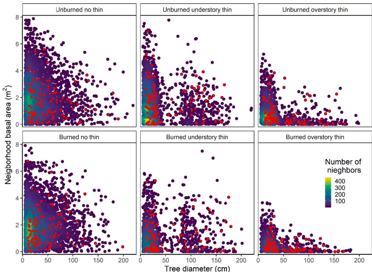
Fig. 1. Sampled trees (red circles) in relation to all live tree diameters and local (10 m) neighborhood basal area within each treatment combination. Unsampled trees colored by density of observations (number of neighbor trees in two dimensional sample space, with lighter regions (yellow) indicating greater number of trees).
