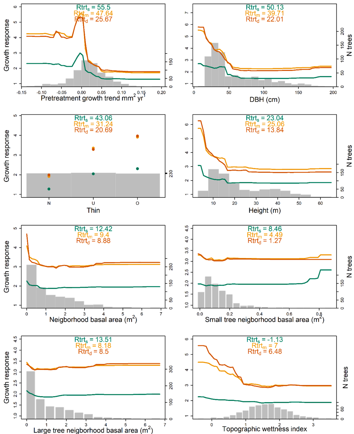
Fig. 6. Partial dependency plots showing relationships between each predictor variable and growth responses metrics in random forest models. Short-term growth response to treatment ( Rtrt_s , green), mid-term growth responses to treatment ( Rtrt_m , orange), and growth response to treatment during drought ( Rtrt_d , red). Numbers within each panel show variable importance values by growth responses metric. Solid lines show trends in growth response metrics in relation to predictor variables. Histograms (gray bars) show the distribution of values for each predictor variable.
