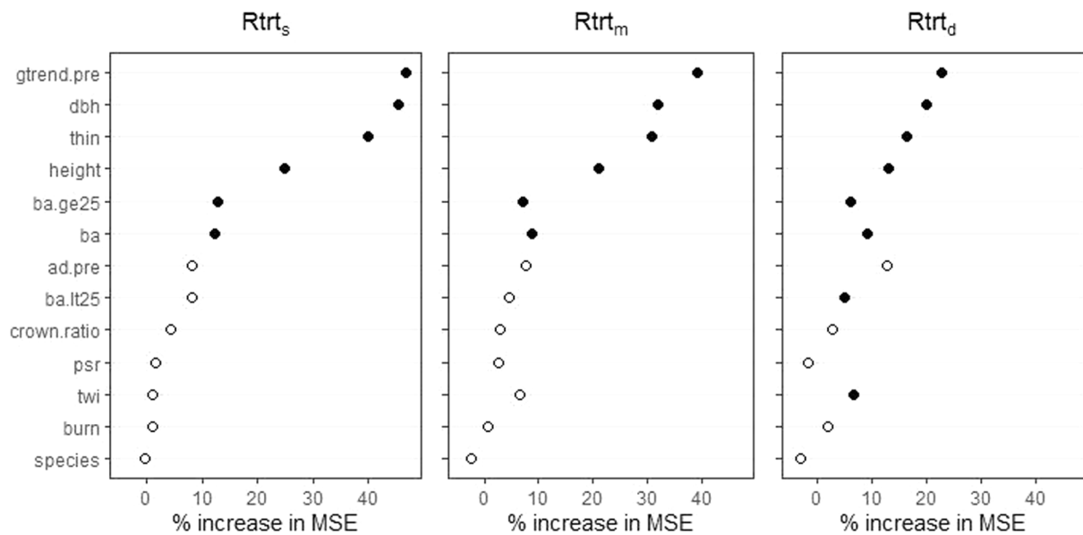
Fig. 5. Variable importance plots for predictor variables from Random Forest (RF) models of growth response metrics. Short-term growth response to treatment ( Rtrt_s , left panel), mid-term growth responses to treatment ( Rtrt_m , center panel), and growth response to treatment during drought ( Rtrt_d , right panel). Variable importance as measure by percent increase in mean squared error (MSE). Solid circles denote variables retained in two-stage variable selection procedures, open circles denote variables removed from the final RF models during variable selection. Predictor variables include pretreatment growth trend (gtrend.pre), diameter (dbh), level of thinning (thin), tree height neighborhood basal area of trees greater than 25 cm dbh (ba.ge25), neighborhood basal area of all trees (ba), neighborhood basal area of trees less than 25 cm dbh (ba.lt25), number of abrupt growth declines prior to treatment (ad.pre), live crown ratio (crown.ratio), potential solar radiation (psr), topographic wetness index (twi), levels of burning (burn), and tree species (species).
