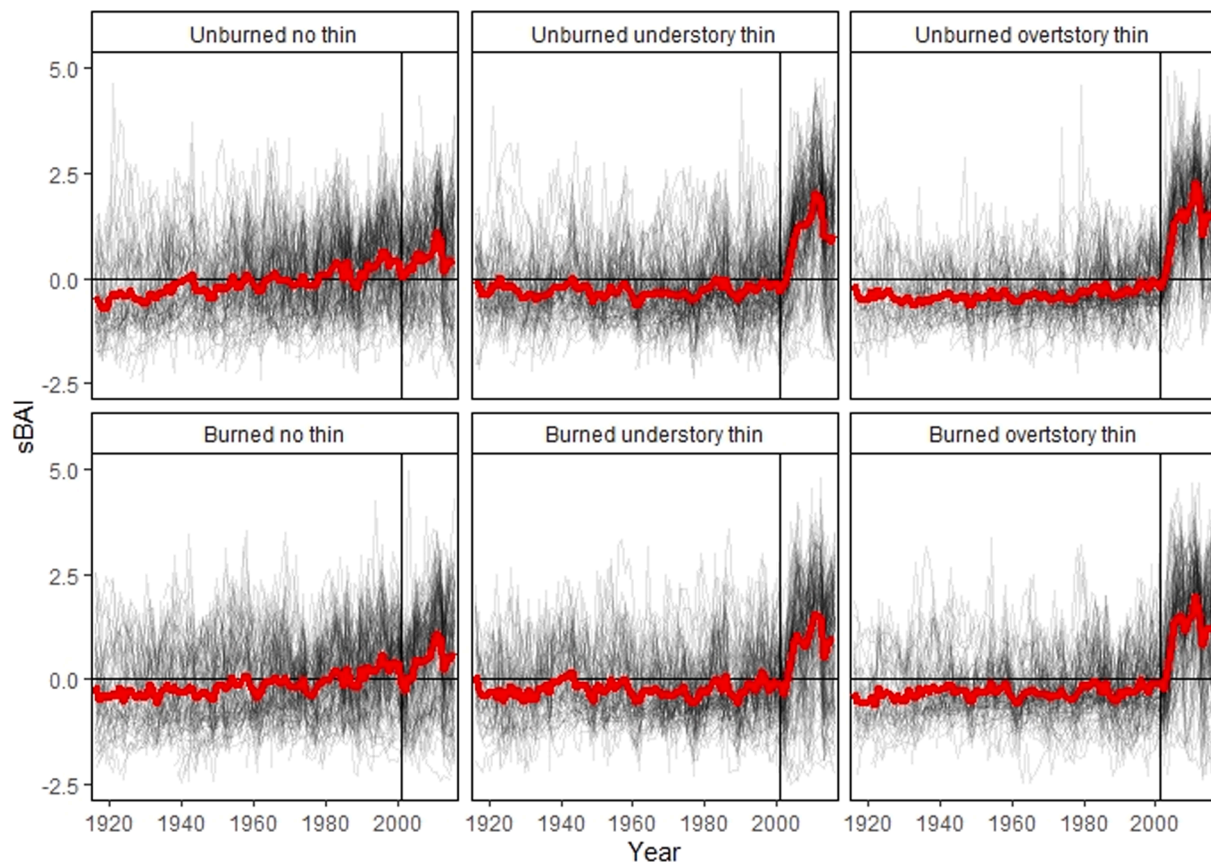
Fig. 3. Growth trends by treatment combination over time. Individual tree (gray lines) and average (red line) are standardized annual basal area increments (sBAI) over time. Vertical black line denotes year of treatment (2001).
