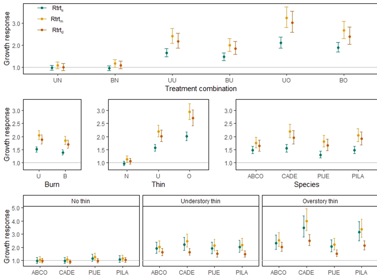
Fig. 4. Estimated marginal means and 95% confidence levels (error bars) of growth responses to burning, thinning, species, burning \times thinning interaction, and species \times thinning interaction. Growth responses greater than 1 denote greater basal area growth versus pretreatment. Growth responses are for short-term after treatment ( Rtrt_s , green), mid-term after treatment ( Rtrt_m , orange), and after treatment during drought ( Rtrt_d , red). Burn treatments were unburned (U) and burned (B). Thinning treatments were no thin (N), understory thin (U), and overstory thin (O). Species were Abies concolor (ABCO), Calocedrus decurrens (CADE), Pinus jeffreyi (PIJA), and Pinus lambertiana (PILA).
