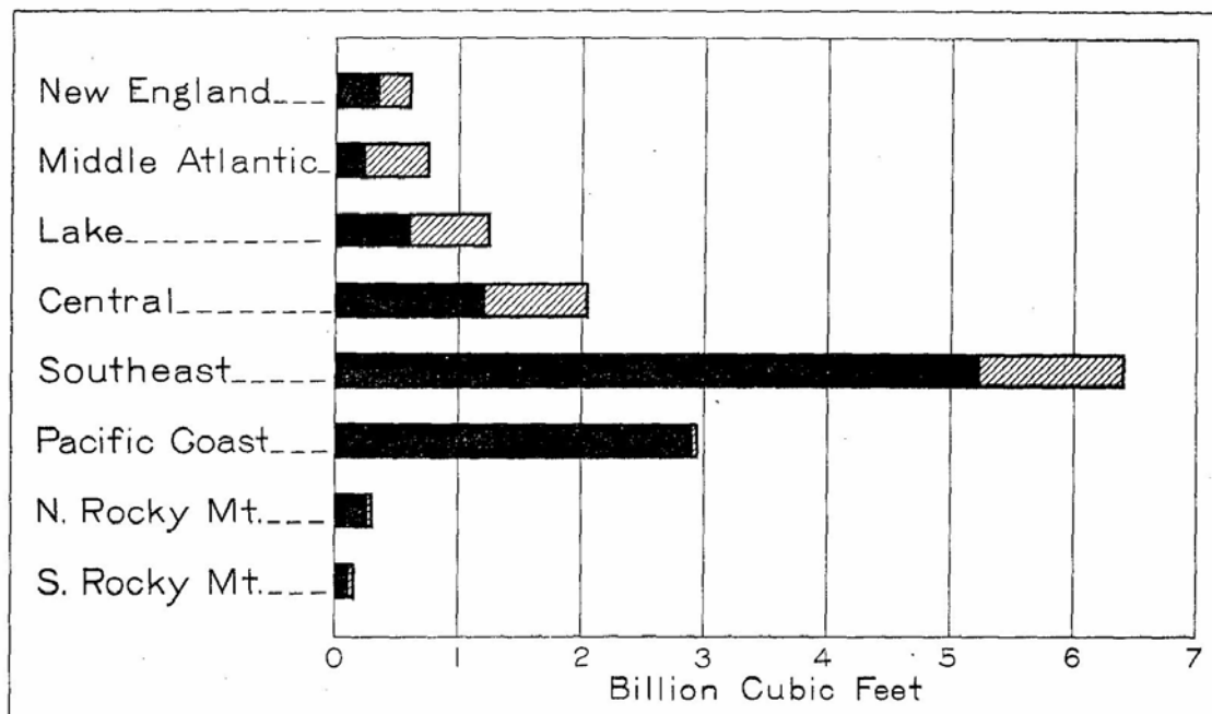
Figure 20.- Total cut on the forests of the United States by tree size and region
