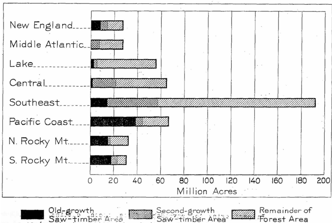
Figure 3. – Old-growth and second-growth saw-timber areas in relation to total forest area of the United States, by region
