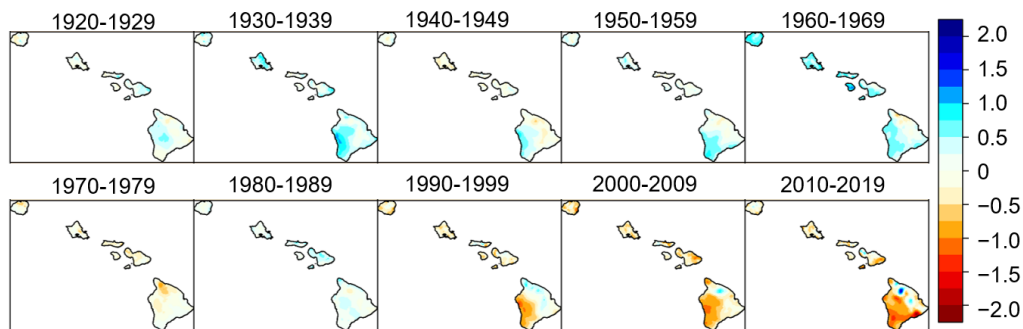
Figure 4. Average 6-month (a) and 12-month (b) SPI by decade (1920–2019) for the State of Hawai'i.
