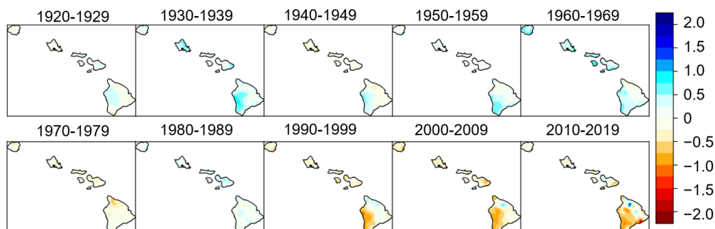
(a) Average SPI-6 by Decade
