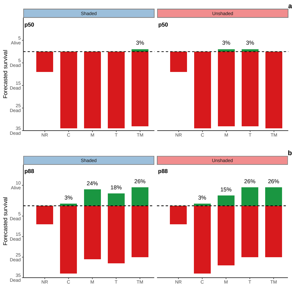
Figure 6. Inferred seedling survival and mortality based on the number of trees in each group with relative water loss < p50 ( RWL \leq 30.13\% ; Panel (a)) and p88 ( RWL \leq 44.24\% ; Panel (b)), based on estimates from Rosner et al. [41]. Green bars and percentages illustrate survival and red bars illustrate mortality.
