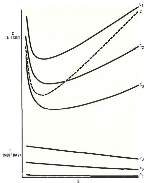
Figure 10.--Total per acre management costs ( C ) and daily production rates ( P ) versus span ( S ) with three classes of aerial systems. ( C and P represent small helicopters, C_2 and P_2 represent large helicopters, C_3 and P_3 represent giant airships, and C is from figure 4.)
