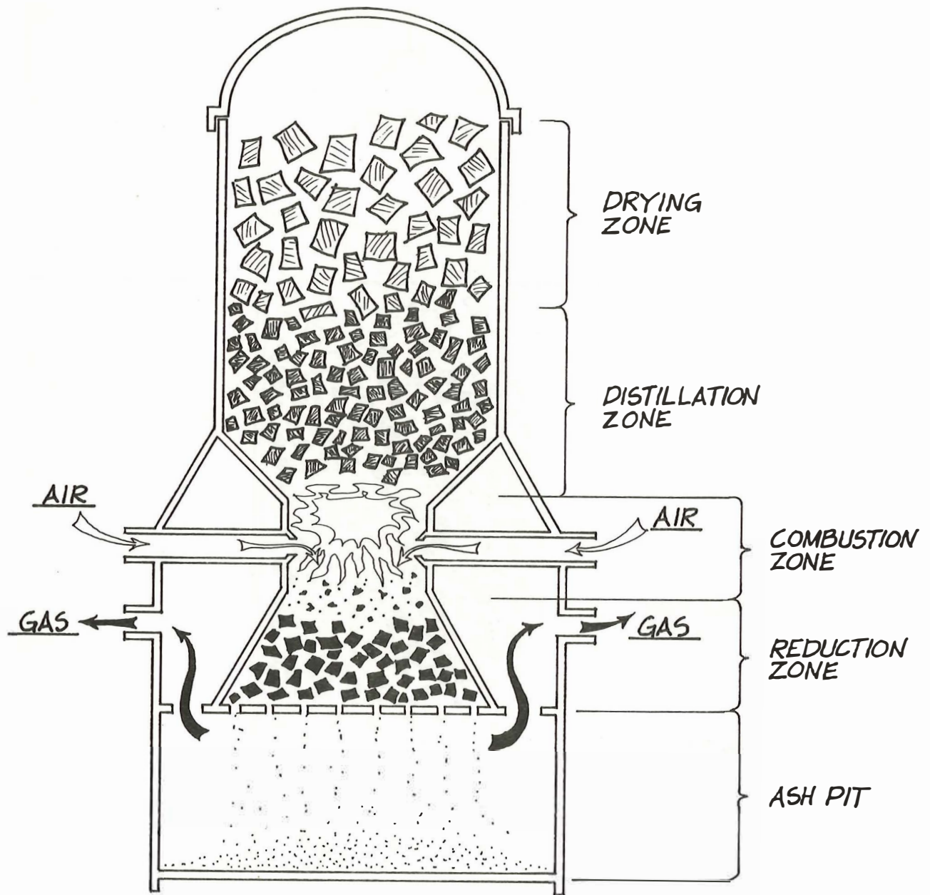
Figure 4.--Downdraft gasifier.
