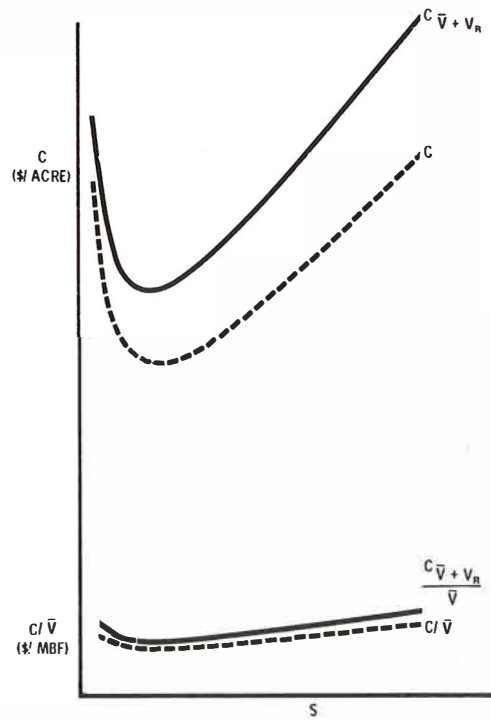
Figure 8.--Effect of residue removal on per acre management cost ( C\bar{V} + \bar{V}_R ) and cost per unit of merchantable volume ( (C\bar{V} + \bar{V}_R)/\bar{V} ) versus span ( S ). ( C and C/\bar{V} are from figure 4.)
