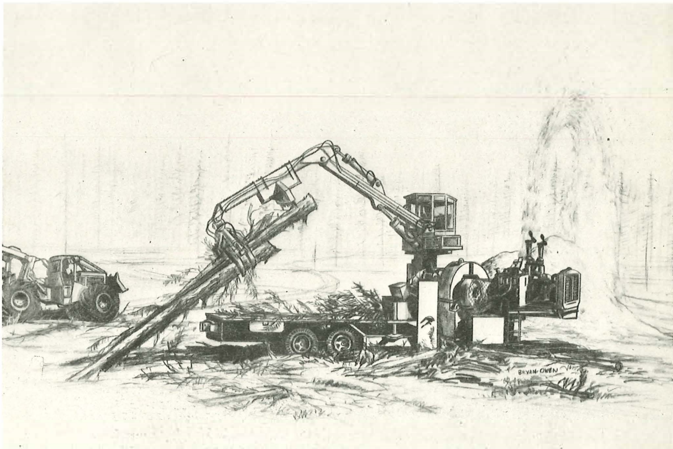
Figure 5.--All material not meeting minimum specifications for saw logs was chipped using a portable whole-tree chipper located on the logging site.
