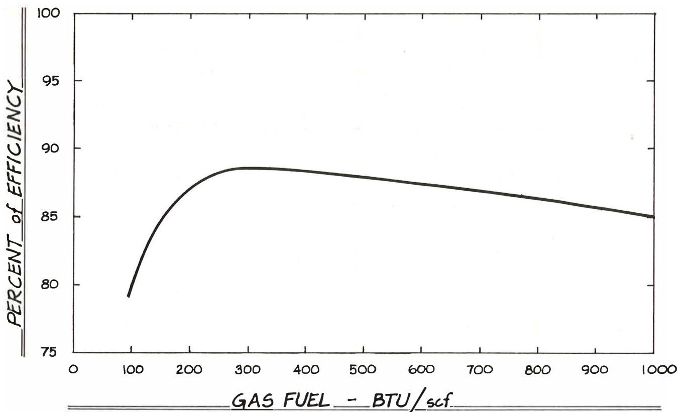
Figure 6.--Gaseous burner efficiencies (Bechtel 1975).
