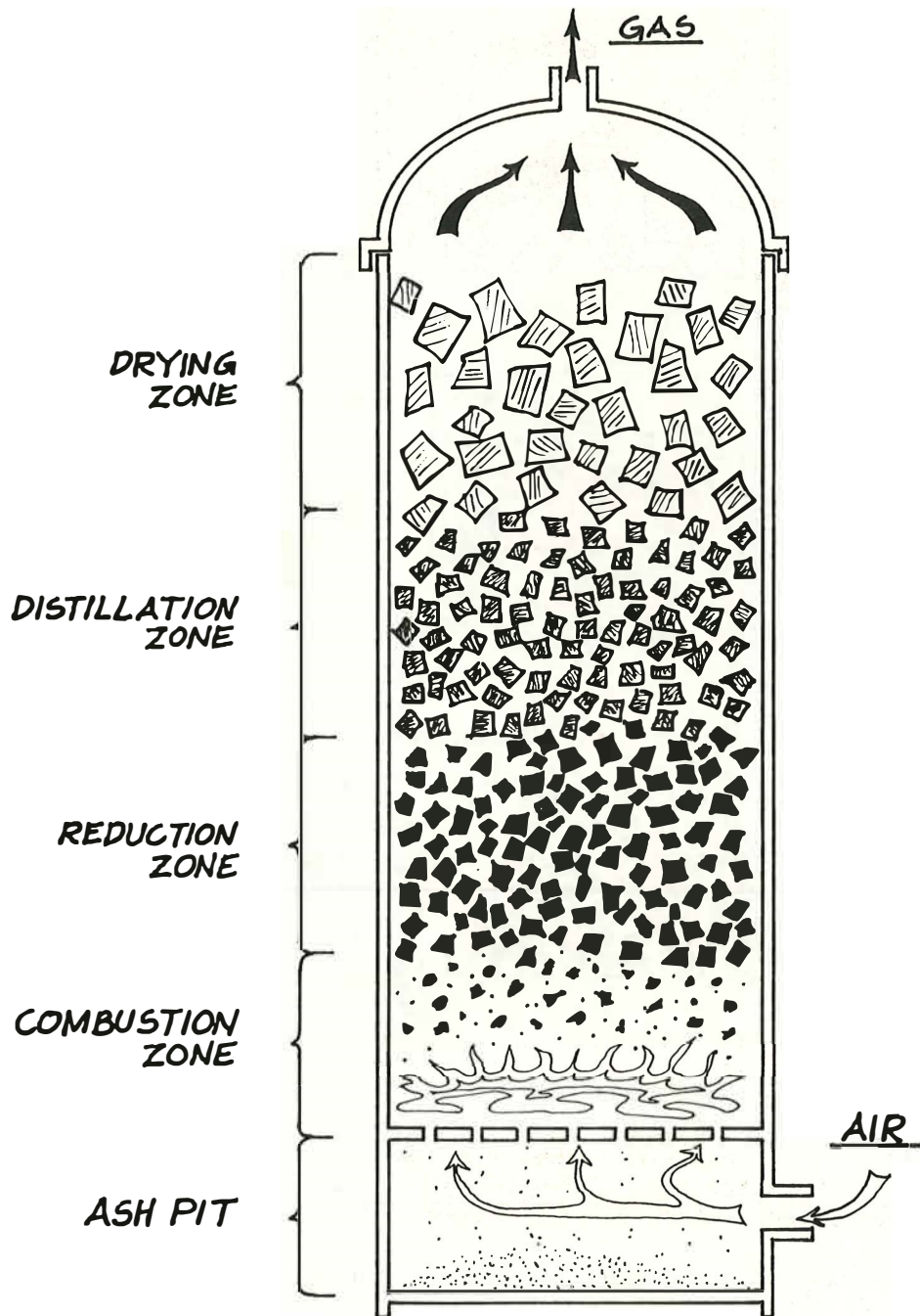
Figure 3.--Updraft gasifier.
