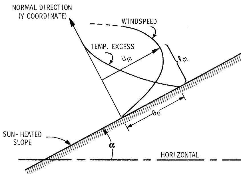
Figure 1.--Windspeed and temperature profiles in the near-surface layer of a sun-heated slope. Note that the y coordinate used to express model results is oriented perpendicular (or "normal") to the sloping surface. The windspeed reaches a maximum ( u_m ) at a distance \ell_m from the surface, while the temperature excess falls from \theta_0 at the surface to zero at a distance of 2\ell_m .
