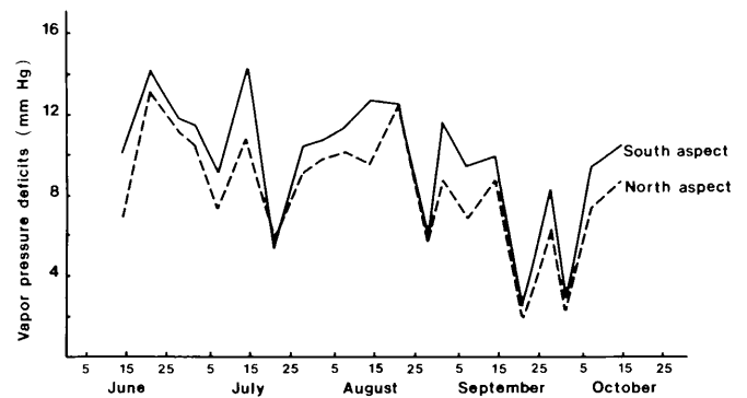
Figure 7.—Comparison of vapor pressure deficits for the 1971 season illustrates the characteristic seasonal pattern between north and south aspects.
