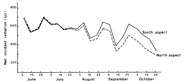
Figure 8.—Comparison of net incident radiation for the 1975 season illustrates the characteristic seasonal pattern between north and south aspects.
