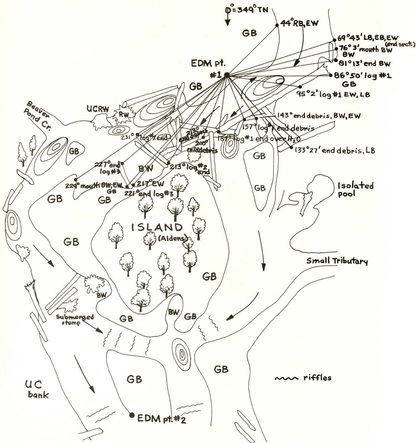
Figure 43—An example of a scale map constructed from data book entries in table 23 for Maybeso Creek.
