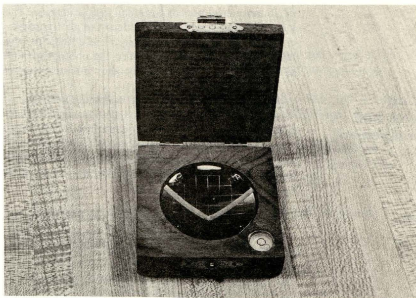
Figure 19—The concave spherical densiometer, model B.
