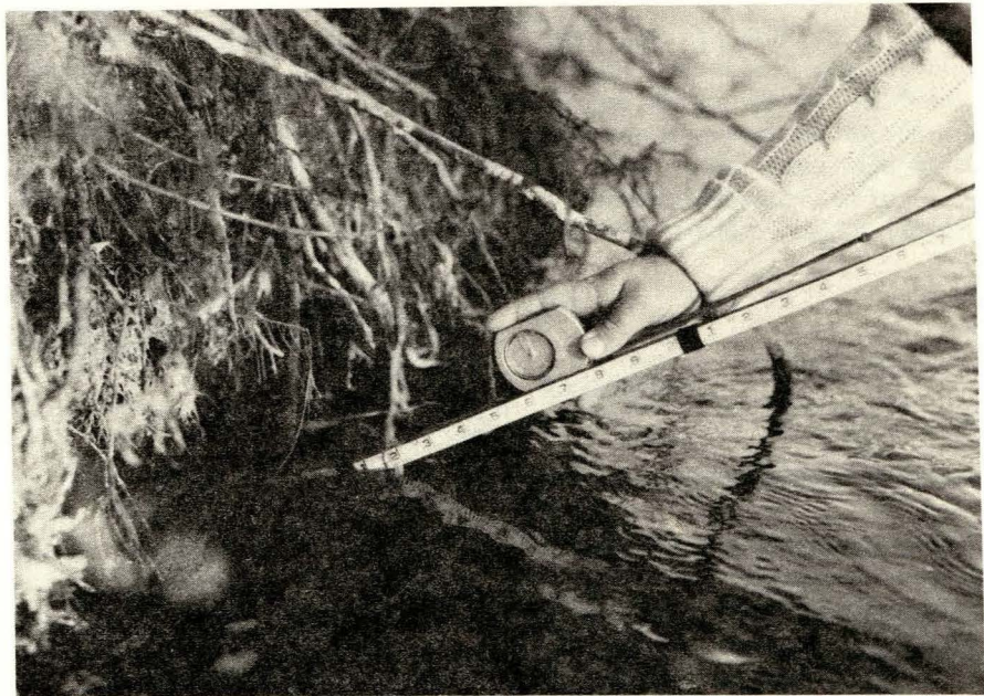
Figure 36—Using a clinometer to measure a bank angle of 45°.
