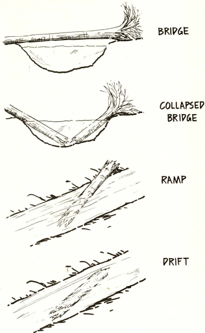
Figure 39—Four categories of large woody debris formations in streams.
