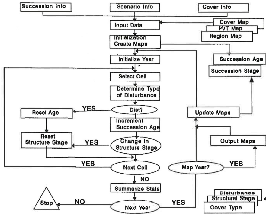
Figure 6—CRBSUM program flow diagram.
