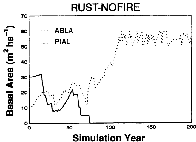
Figure 25 —FIRE-BGC basal area predictions for the RUST-NOFIRE scenario for 200 years of simulation.
