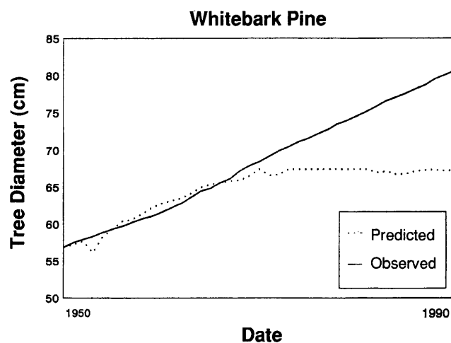
Figure 33 —Predicted and observed diameters (DBH) for a whitebark pine tree.
