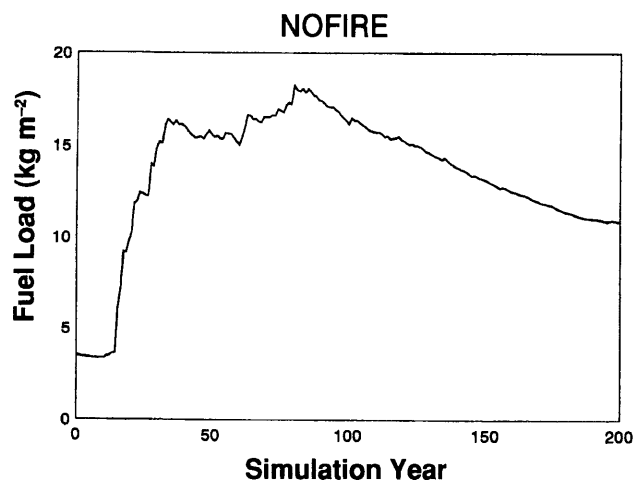
Figure 28 —Predicted woody fuel loadings for the NOFIRE scenario using FIRE-BGC. Loadings are for all size classes of woody fuels (1, 10, 100, 1,000 hour fuel classes).
