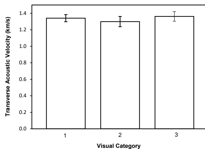
Figure 7. Mean transverse stress wave velocities (km/s) by visual category. Error bars represent a 95% confidence interval.
