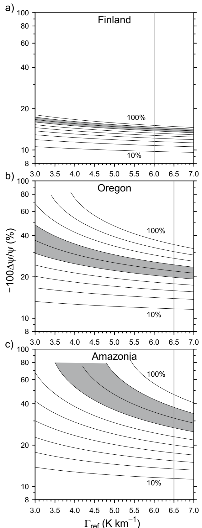
Fig. 3 Relative decrease (%) in the propensity of cold-air drainage index ( \psi ) by 2100 CE (RCP8.5) as a function of the reference lapse rate \Gamma_{\text{ref}} for the a Finland, b Oregon, and c Amazonia sites. Solid lines are contours of constant RH ranging from 10 to 100% in 10% increments, increasing upward in the panel. The shaded area shows the representative RH range for each site. The vertical gray line marks the value of \Gamma_{\text{ref}} used for Fig. 2. See Table 1 for reference conditions and projected changes in conditions assumed at each site
