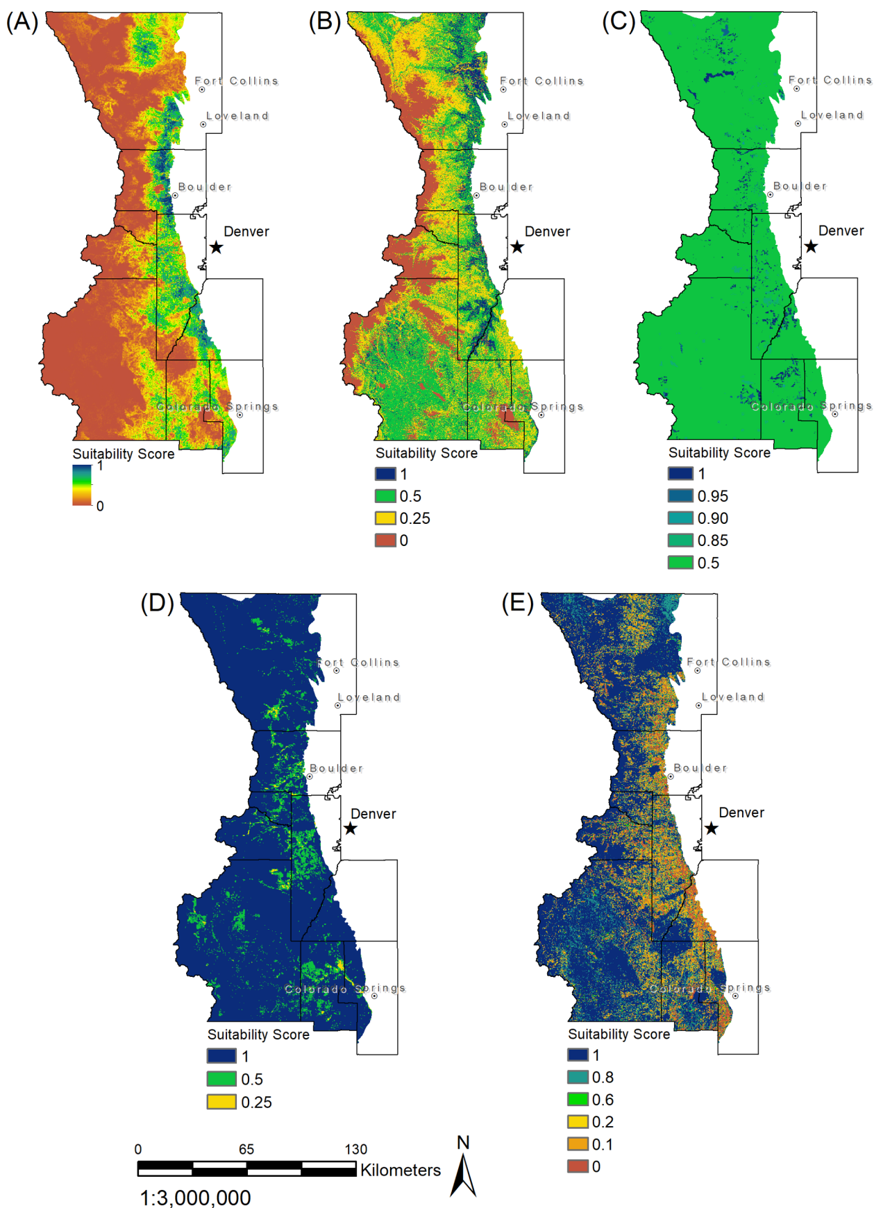
Fig. 2. Individual suitability layers used to determine overall suitability for broadcast prescribed fire on the Front Range, including (A) wildfire hazard (WH), (B) vegetation types, fuels, and areas of historical low-severity fire (VFH), (C) existing treatment areas (T), (D) wildland-urban interface (WUI), and (E) prescribed fire behavior (PFB).
