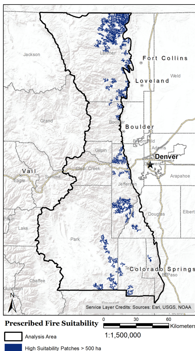
Fig. 5. High suitability patches for prescribed fire greater than 500 ha in size on the Front Range.
