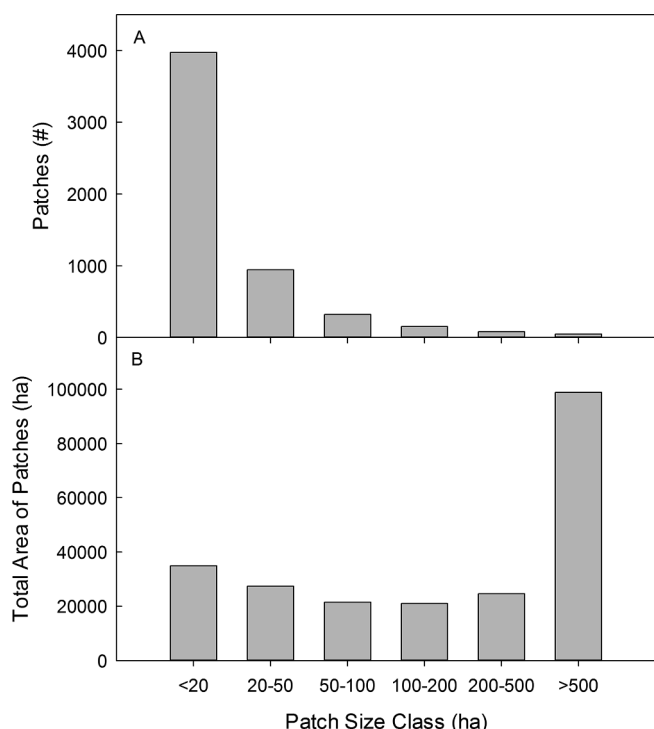
Fig. 4. (A) Number and (B) total area (ha) of high suitability patches for prescribed fire by patch size class on the Front Range. High suitability patches were determined using the 4-neighbor rule in Fragstats, whereby high suitability pixels adjacent in one of the cardinal directions were grouped together to define patches of high suitability.
