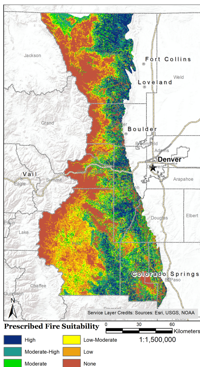
Fig. 3. Overall suitability for broadcast prescribed fire on the Front Range based on wildfire hazard, vegetation types, fuels, and areas of historical low-severity fire, existing treatment areas, wildland urban interface, and prescribed fire behavior.
