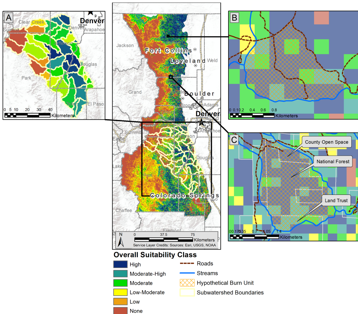
Fig. 6. Example applications of prescribed fire suitability output: (A) the suitability layer can be scaled to other planning units such as sub-watersheds and used in comprehensive forest management planning efforts to help identify treatment priorities based on opportunities for prescribed fire; (B) the suitability layer can be combined with containment features layer (e.g., roads and water features) to delineate individual burn units within a single land ownership; and (C) the suitability layer can facilitate cross-boundary and interagency planning of prescribed fire projects to avoid creating holding lines that coincide with property boundaries but rather are tied to landscape features.
