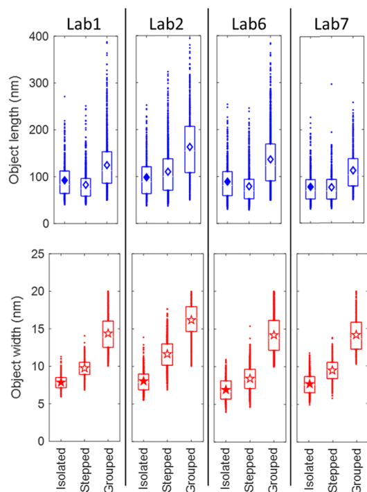
Fig. 10 Size measurements of isolated CNCs, stepped CNCs and grouped CNCs. Object length and widths are estimated by the major and minor axis length of the oval encapsulation of the given object, respectively. Diamond and star markers represent mean values for each group, with filled symbols for the isolated CNCs. Upper and lower edges of the vertical rectangles correspond to the 75th and 25th quartiles for each group
