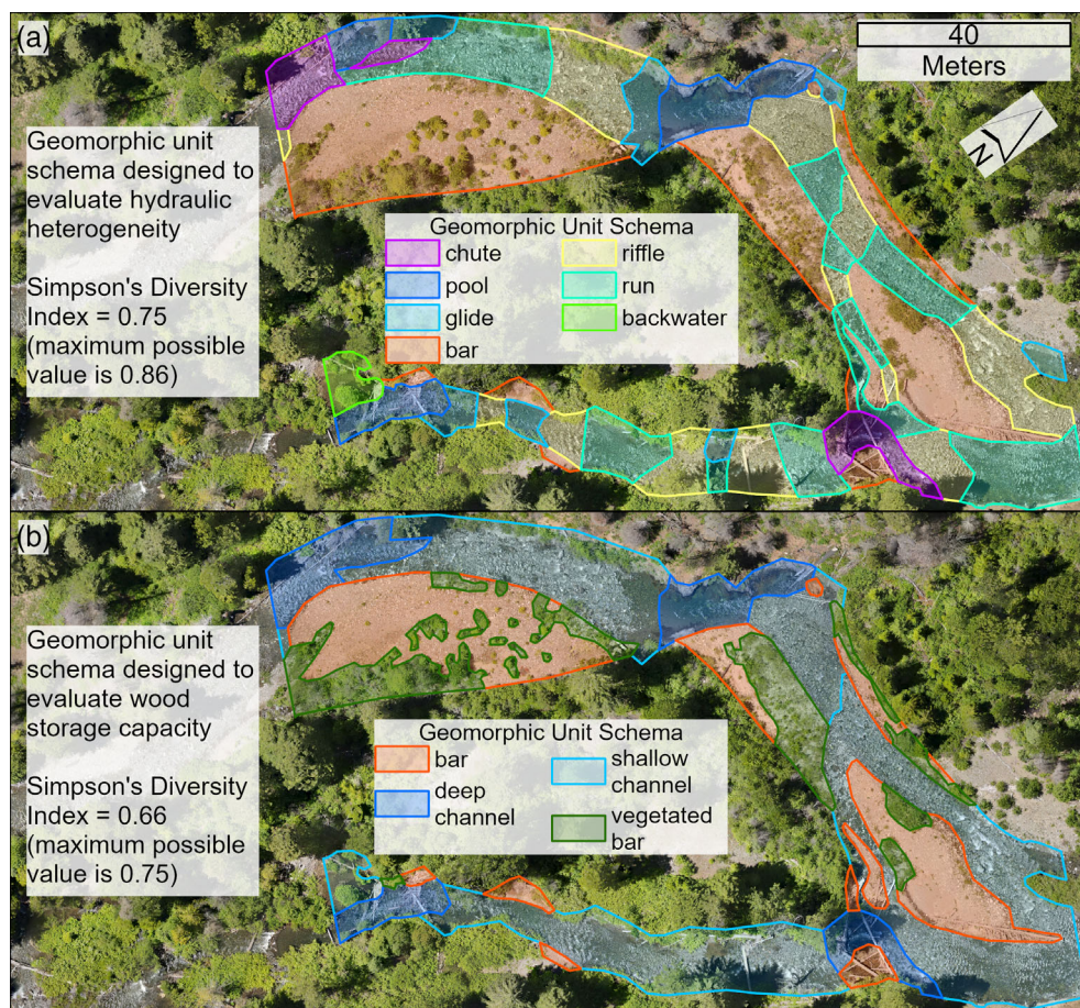
FIGURE 1 The North Fork Teanaway River, WA, USA shows how different geomorphic unit schemas produce different degrees of heterogeneity, even over the same area and using the same metric. Diversity indices computed for the same area will produce different values based on a hydraulic heterogeneity-focused schema (a) versus a wood storage capacity-focused schema (b), and those values are not meaningfully comparable [Color figure can be viewed at wileyonlinelibrary.com ]
