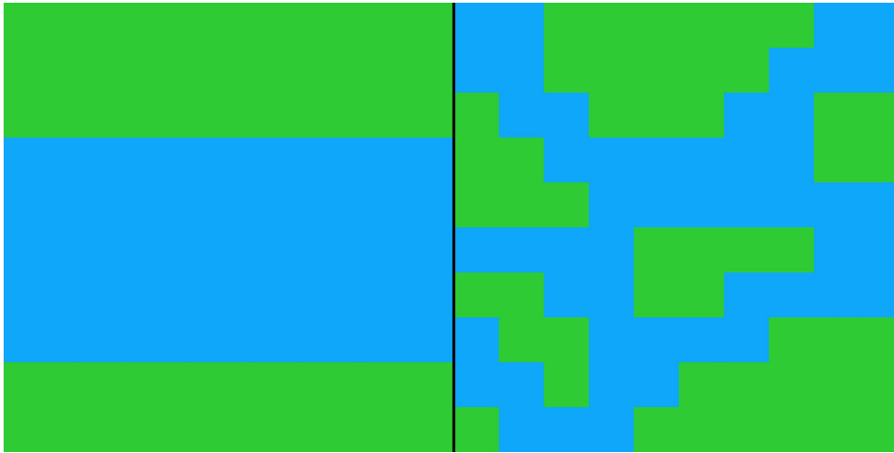
FIGURE 2 Two hypothetical landscapes with identical evenness (50 blue/darker squares, 50 green/lighter squares), but very different spatial configuration [Color figure can be viewed at wileyonlinelibrary.com ]
