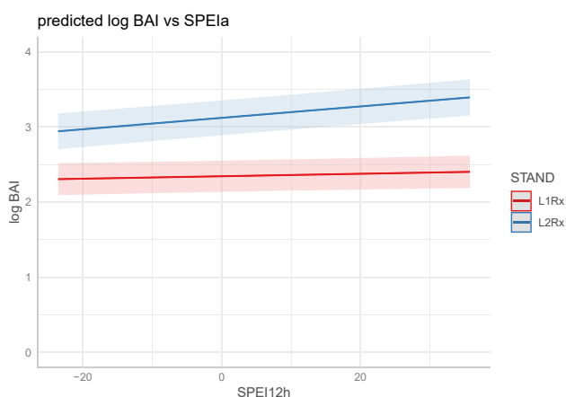
Fig. 8. Interaction of SPEI12h with stand in L1Rx vs. L2Rx comparison. The coefficients of SPEI12h were significantly different at the two sites; L2Rx was more responsive to SPEI12h. Upper line represents L2Rx stand.
