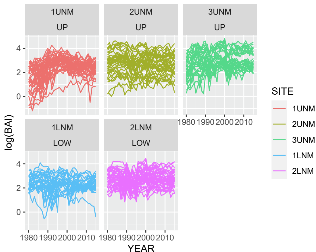
Fig. 4. Traces of log(BAI) trees in lowland and upland no management stands (LNM, UNM).
