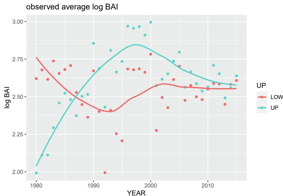
Fig. 5. Observed average log(BAI) for upland (UNM) and lowland (LNM), no management stands with smooth spline. Upper fitted curve represents upland trees.
