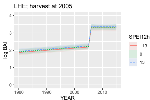
Fig. 7. Piecewise linear models. Left: Predicted log(BAI) at LHE to show response to treatment without smoothing. Right: log(BAI) for piecewise linear model (lines). The dots represent the observed average log(BAI) in L1Rx. In both graphs SPEI12h has average value 0, and standard deviation \sim 13 .
