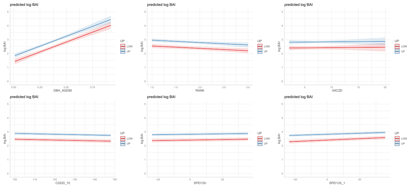
Fig. 3. Effect plots for covariates for unmanaged upland (UNM) and lowland (LNM) stands. Predicted log(BAI) is shown when setting all other variables to their average values. Upper line represents upland trees in all graphs.
