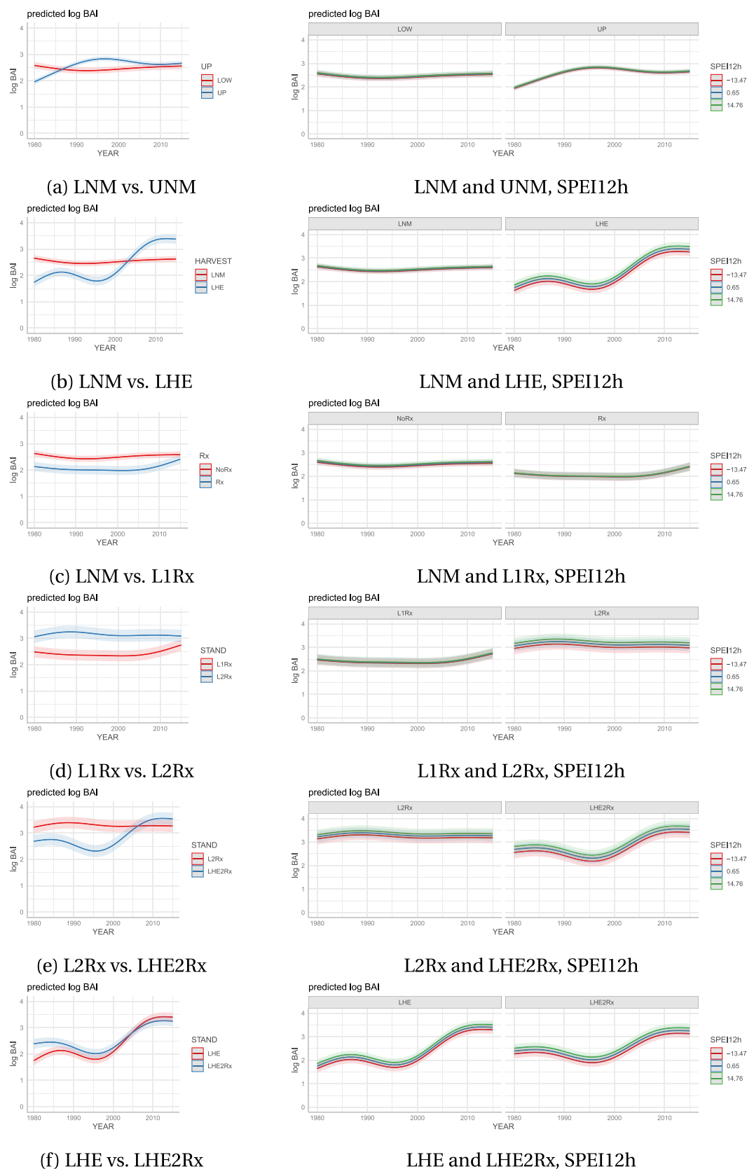
Fig. 6. Paired comparisons between predicted BAI of (a) lowland unmanaged (LNM) and upland unmanaged (UNM) trees; (b) LNM and lowland even harvest trees (LHE); (c) LNM and lowland one prescribed fire trees (L1Rx) (d) lowland one and two prescribed fire trees (L1Rx, L2Rx) trees; (e) L2Rx and LHE2Rx; and (f) LHE and LHE2Rx trees.
