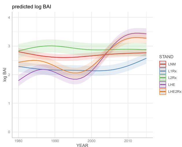
Fig. 9. Predicted values of BAI for all lowland stands. Dates when treatments were imposed are given in Table 1.
