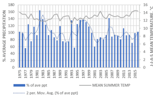
Fig. 2. Annual % of average precipitation (bars), summertime (June, July, August, September) mean air temperature (grey line), and 2-yr moving average precipitation (dotted line). Data is from PRISM.
