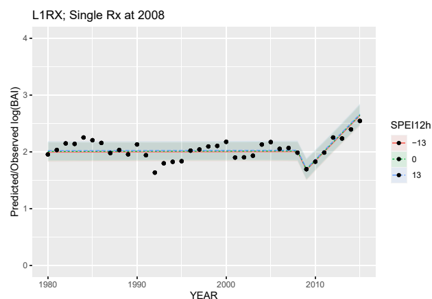
Fig. 7. Piecewise linear models. Left: Predicted log(BAI) at LHE to show response to treatment without smoothing. Right: log(BAI) for piecewise linear model (lines). The dots represent the observed average log(BAI) in L1Rx. In both graphs SPEI12h has average value 0, and standard deviation \sim 13 .
