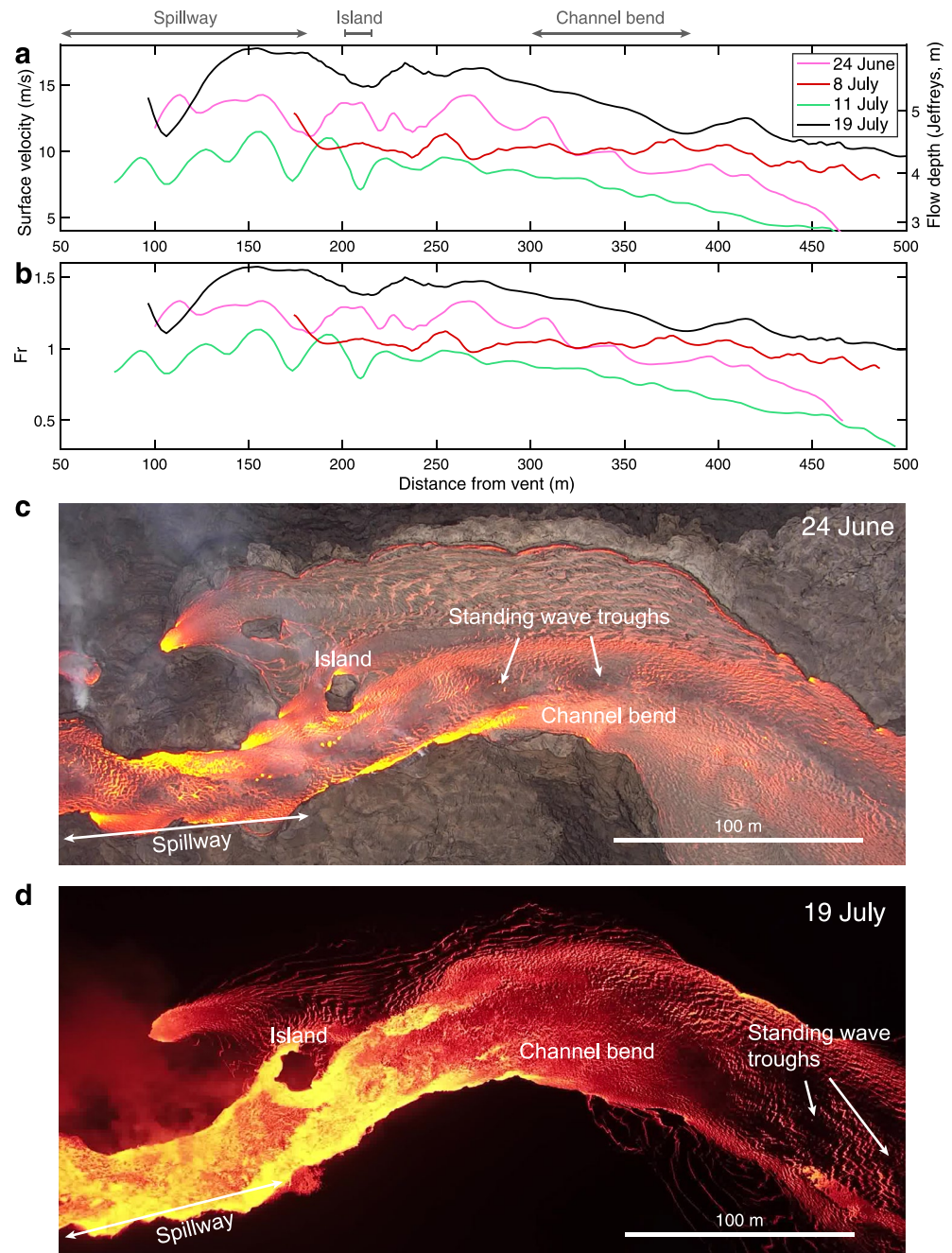
Figure 9. (a) Maximum surface velocity and derived flow depth along proximal channel reach. (b) Froude (Fr) number calculated from depth estimates based on Jeffreys' Equation 6. (c and d) Annotated examples of UAS video frames from 24 June and 19 July (surge) for reference.
