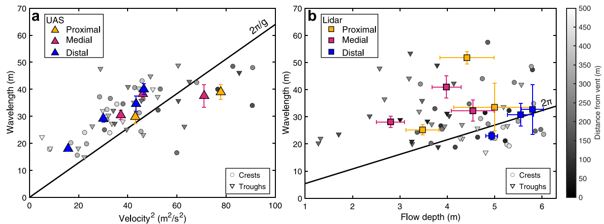
Figure 10. (a) Test of the Kennedy (1963) scaling ( 2\pi/g line) for the relation between wavelength and velocity. L_t and L_c are plotted relative to the square of the mean flow velocity ( U in Equation 2). Grayscale in both plots represents the distance from the vent. Averages are shown for the proximal (<200 m; spillway), medial (150–300 m; wider zone with best wave morphology), and distal (>350 m; after the channel bend) sections of the reach for each survey date. (b) Testing the Kennedy (1963) relationship ( 2\pi line; Equation 3) with DEM measurements of flow wavelength and depth. L_t and L_c are plotted relative to depth from lidar differencing.
