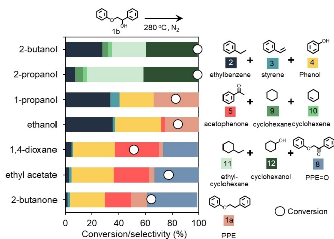
Figure 3. Cleavage of the \beta -O-4 bond of 2-phenoxy-1-phenylethanol (PPE-OH, 1b) by Ru/C in selected protic and aprotic polar solvents. Reaction condition: 280 °C, 4 h, 8 bar N_2 , 1 wt.% 2-phenoxy-1-phenylethanol/solvent, 20 wt.% catalyst loading.
