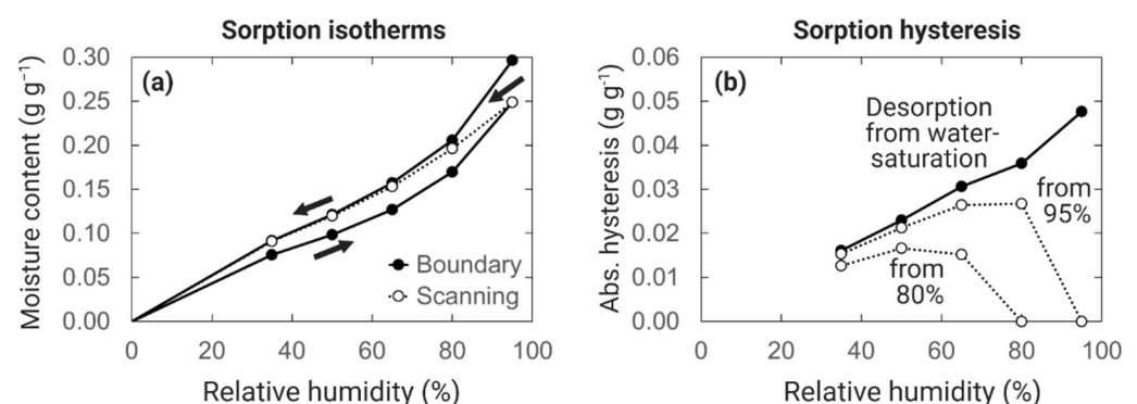
Figure 6. (a) Moisture sorption isotherms, and (b) absolute hysteresis curves for wood of Norway spruce [174]. Desorption isotherms are determined either from full water saturation (boundary curves) or from conditioning in absorption to either 95% or 80% RH (scanning desorption).
