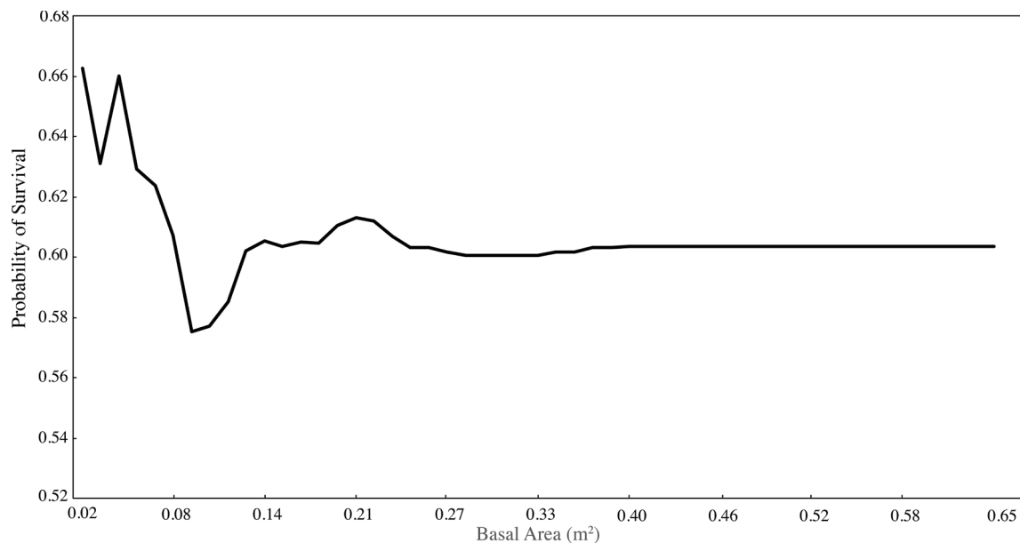
Fig. 5. Partial dependence plot estimating the probability of survival as influenced by individual-tree basal area ( \text{m}^2 ) following a November 2018 intermediate-severity wind disturbance in Savage Gulf State Natural Area, TN, USA. Partial dependence plot depicts the influence of basal area ( \text{m}^2 ) on the likelihood of tree survival based on balanced random forest classification algorithm when all other predictor variables are held constant.
