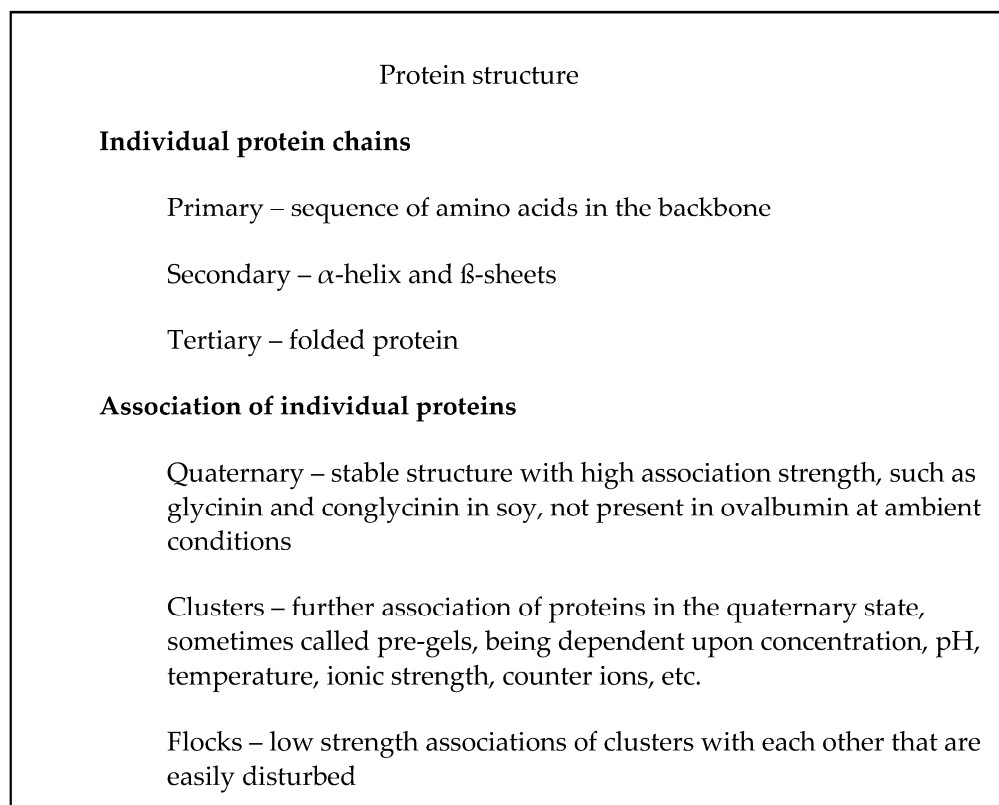
Figure 18. Levels of protein structure from the strong amino acid backbone to the weak flocks.
