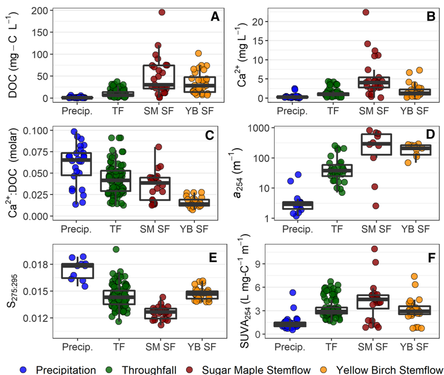
Fig. 2 Boxplots and jitter plots of A dissolved organic carbon (DOC), B \text{Ca}^{2+} , C the molar ratio of \text{Ca}^{2+} to DOC, D Napierian absorbance coefficient at 254 nm ( a_{254} ), E absorbance spectra slope from 275 to 295 nm ( S_{275:295} ), and F specific UV absorbance at 254 nm ( \text{SUVA}_{254} ) across flow paths. Boxes depict the median and first and third quartiles. Whiskers extend to the minimum or maximum value no further than 1.5 times the inner quartile range
