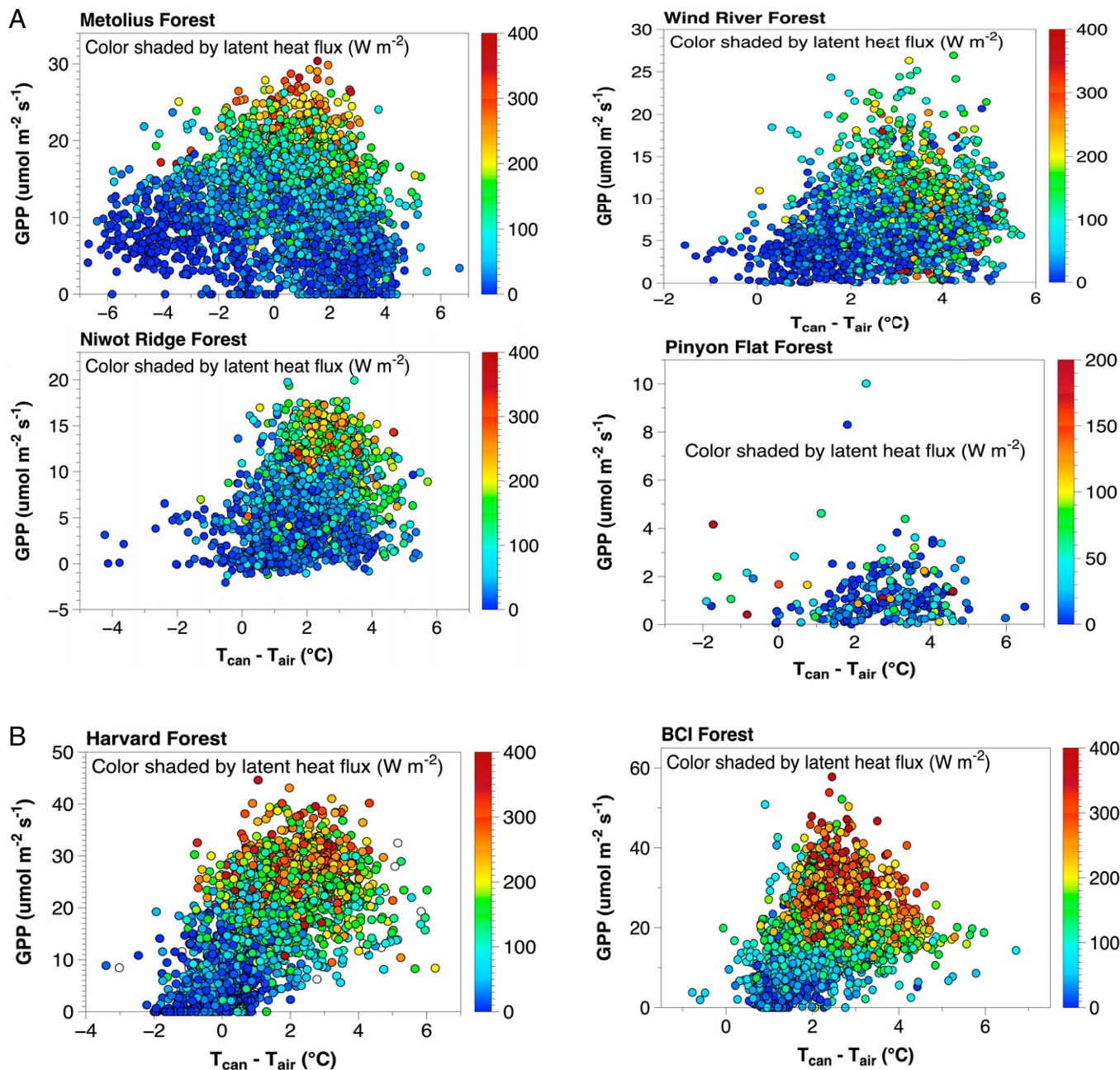
Fig. 4. Relationship between gross \text{CO}_2 uptake ( \text{GPP} , \mu\text{mol m}^{-2} \text{s}^{-1} ) and T_{\text{can}} - T_{\text{air}} ( ^{\circ}\text{C} ) at needleleaf-dominated sites (Metolius, Wind River, Pinyon Flat, and Niwot Ridge, A) and broadleaf-dominated sites (Harvard, BCI, B). The color bar legend represents the latent heat flux ( \text{W m}^{-2} ).
