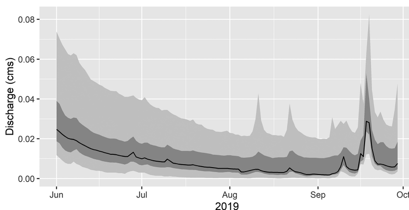
FIGURE 7 Estimated mean daily discharge (cubic meters per second; cms) across study sites during the study period, 1 June 2019 to 30 September 2019, with 50th (black curve) and 25th to 75th (dark grey band) percentiles and minimum and maximum (light grey band) discharge
