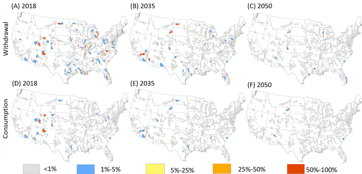
Fig. 6. Ratio of fossil fuel-fired power plants' water withdrawal (top) and consumption (bottom) in 2018, 2035, and 2050 to compared to average (2001–2015) natural streamflow conditions. Subbasins without a fossil fuel-fired power plant are shaded gray. Fossil fuel-fired power plants in the majority of the subbasins withdraw and consume only a small portion of the available water within the subbasin. Around 5% subbasins were identified to withdraw more than 1% of the streamflow available within the subbasin.
